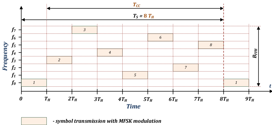
Figure 4. Diagram of the fast frequency hopping technique for an example code sequence pattern of length 8 ( T_S = 8 \cdot T_H ).
