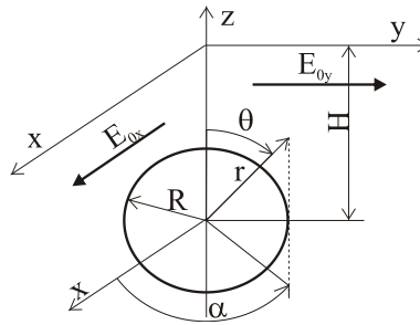
Fig. 1. Sphere in uniform electric field
