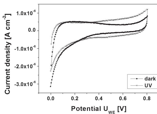
Fig. 11. Cyclic voltammograms obtained for photocatalyst deposited at 15 mA cm -2 in dark and under UV irradiation.
