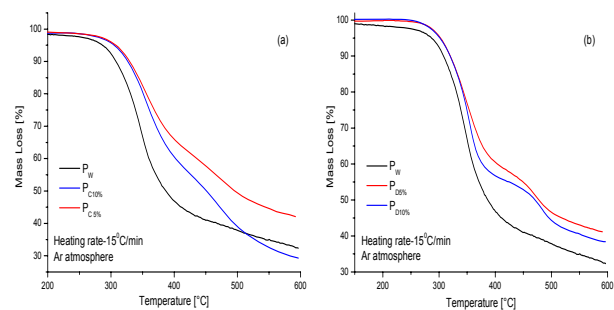
Fig. 3: Thermogravimetric analysis (TGA) of control PUFs (P W ): a) and foams modification by Cloisite®10A in 5 and 10 %wt. (P C 5% and P C 10%); b) foams modification by decabromodiphenyloxid in 5 and 10 %wt. (P D 5% and P D 10%)
