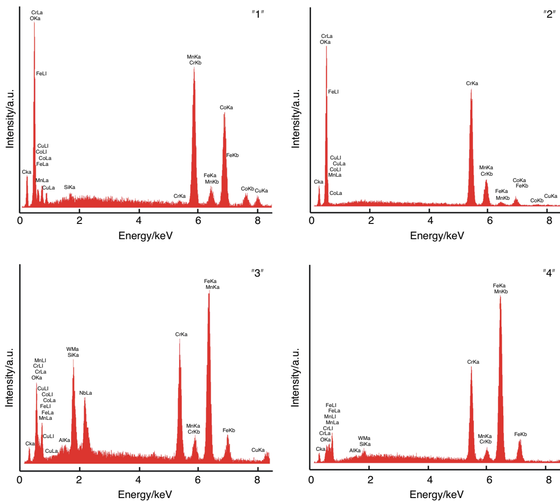
Fig. 11 SEM micrograph of the Crofer 22 H/Mn 1.45 Co 1.45 Cu 0.1 O 4 layered system after 1200 h of cyclic oxidation in air at 800 °C, with EDS point analysis spectra recorded for regions marked "1", "2", "3" and "4" in the micrograph
