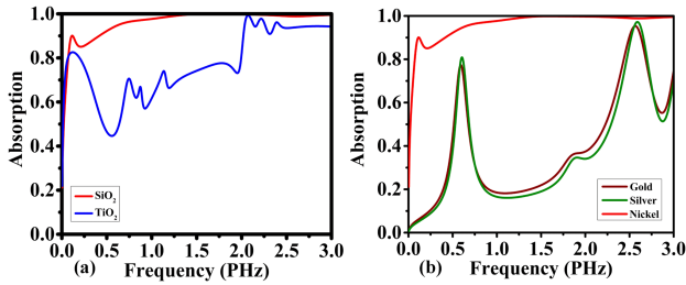
Fig. 4. Absorption spectra of the proposed design under varying substrate and resonator material conditions: (a) Absorption spectra under different substrate materials, and (b) absorption spectra under different resonator materials.
