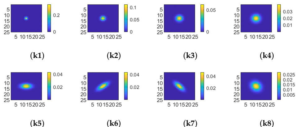
Figure 3. Blur kernels.
