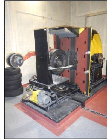
Fig.6. Roadwheel facility.
