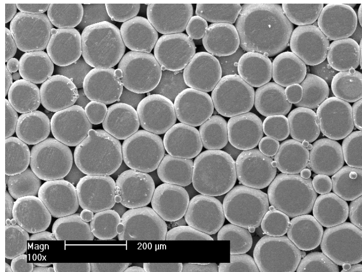
Fig. 3. Surface microstructure (SEM) of the sample after the compacting powder obtained by plasma spraying method
