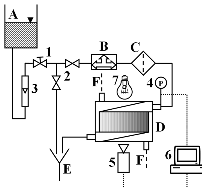
Figure 1: Diagram of experimental rig, elements of the flow system: A – water tank, B – air separation system, C – filter, D – test section, E – outflow, F – section heating/cooling facility; elements of the control and measuring system: 1 – control valve, 2 – cut-off valve, 3 – rotameter, 4 – pressure transducer, 5 – fast shutter speed camera, 6 – synchronization and data acquisition system, 7 – light source.
