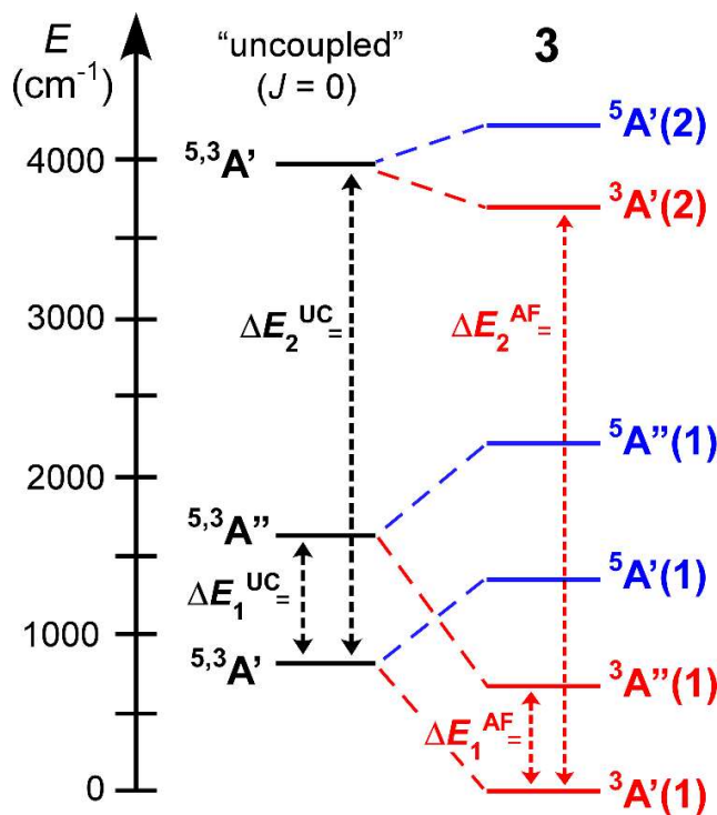
Figure 10. Right: CASSCF/NEVPT2 computed energies of the six lowest-energy states of complex 3 . Energy splittings between the three triplet states are indicated by \Delta E_1^{\text{AF}} and \Delta E_2^{\text{AF}} (AF = antiferromagnetic). Left: Relative energies of ligand-field states in the absence of exchange coupling between Co(II) and \text{L}^{\text{O,N}}\text{ISQ} (i.e., J -value of zero). The energy of each uncoupled (UC) state was calculated by taking the weighted average of the corresponding quintet and triplet energies: E^{\text{UC}} = 3/8 E(\text{triplet}) + 5/8 E(\text{quintet}) .
