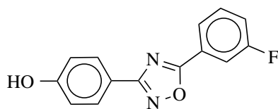
4-(5-(3-Fluorofenylo)-1,2,4-oksadiazol-3-ilo)fenol 32b
