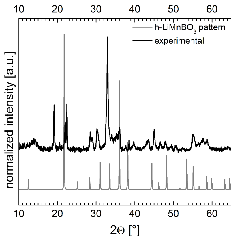
Fig. S2: Comparison of XRD pattern taken after 20 h of annealing at 525 °C (black) with h-LiMnBO 3 simulated pattern (grey).
