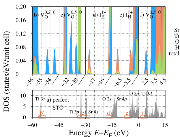
Figure 12. Influence of the V_{\text{O}} and I_{\text{H}} defects on the electronic structure of STO. Panel (a) (bottom) presents the total DOS of perfect STO and serves as a guide. It indicates the position of regions shown in panels (b–f), which present features introduced by V_{\text{O}}^{0,S=0} (b,c,f) and I_{\text{H}}^{1+} (d,e) defects in the low-energy parts (b–e) and within the forbidden gap (f). Panels (b–f) present the local (atom-decomposed) DOS. All panels use the same reference energy ( E_{\text{F}} of perfect STO).
