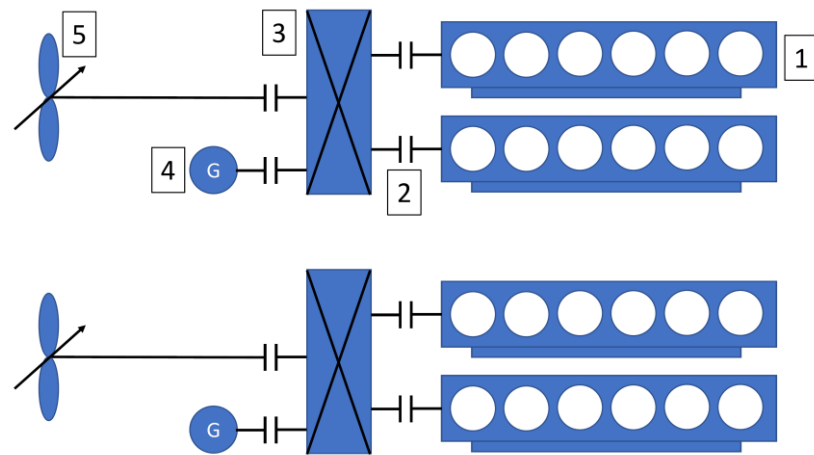
Figure 5 Typical Great Lakes 1000ft self-unloader's propulsion system layout (description in text)
