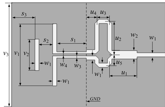
FIGURE 6. Geometry of the planar Yagi antenna [66].
