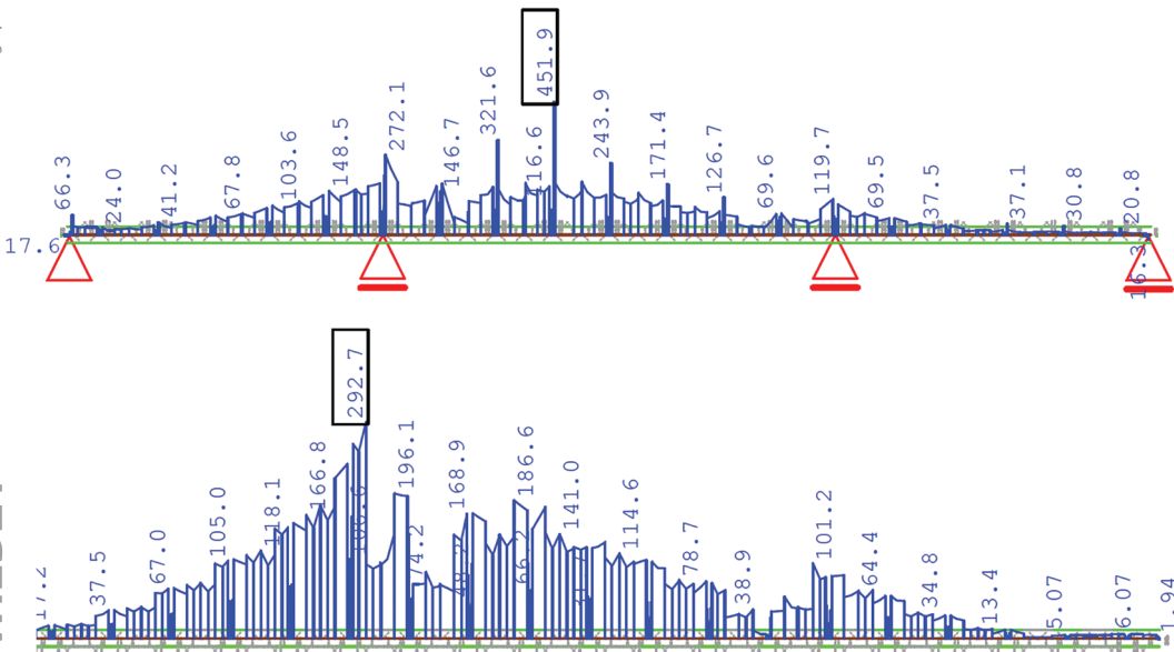
Figure 22. Chosen results of the FEM structural analysis: maximal stress H MH for external girder – lower and upper chords
