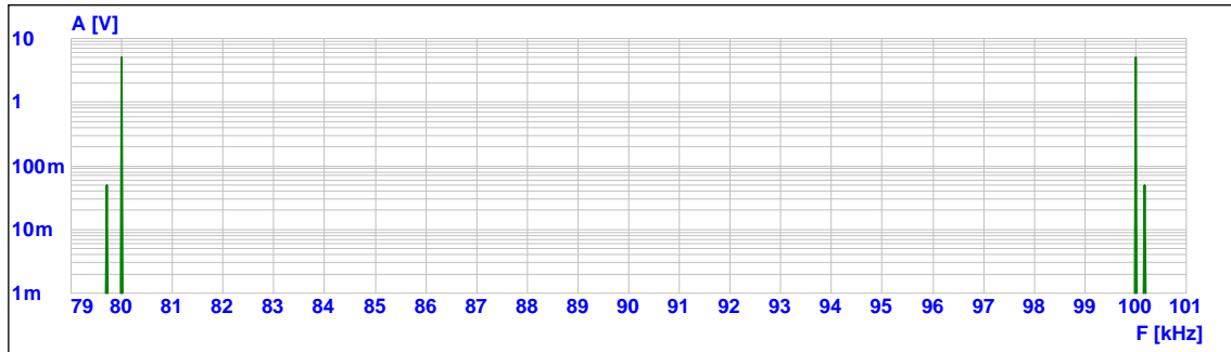
Fig. 6. The spectrum of hydrophone signal being amplified for G=60\text{dB} :
