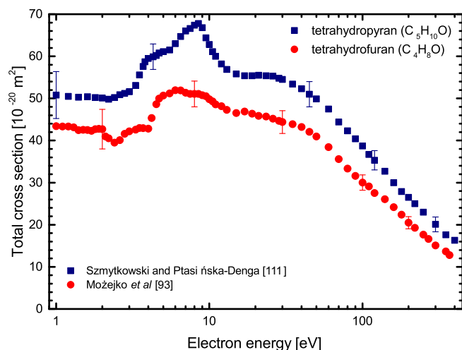
Fig. 14. Experimental grand -total cross section for electron scattering from tetrahydropyran ( C_5H_{10}O ): ■ [111]. For comparison TCS for electron scattering from tetrahydrofuran (THF) is also shown: ● [93].
