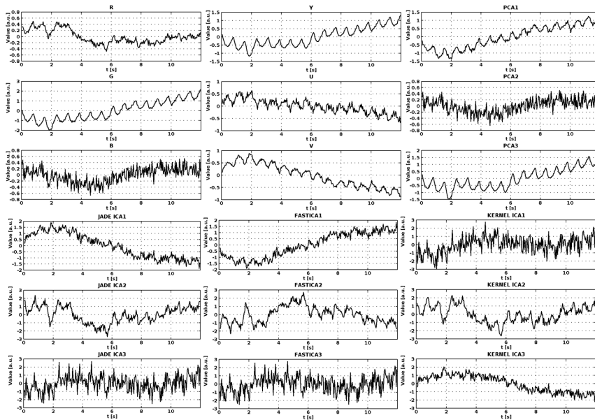
Fig. 3. An example of pre-processed signals obtained for: (top, from left): a) RGB color model; b) YUV color model; c) PCA components from R , G , B signals; (bottom, from left): JADE ICA, Fast ICA, and KERNEL ICA.
