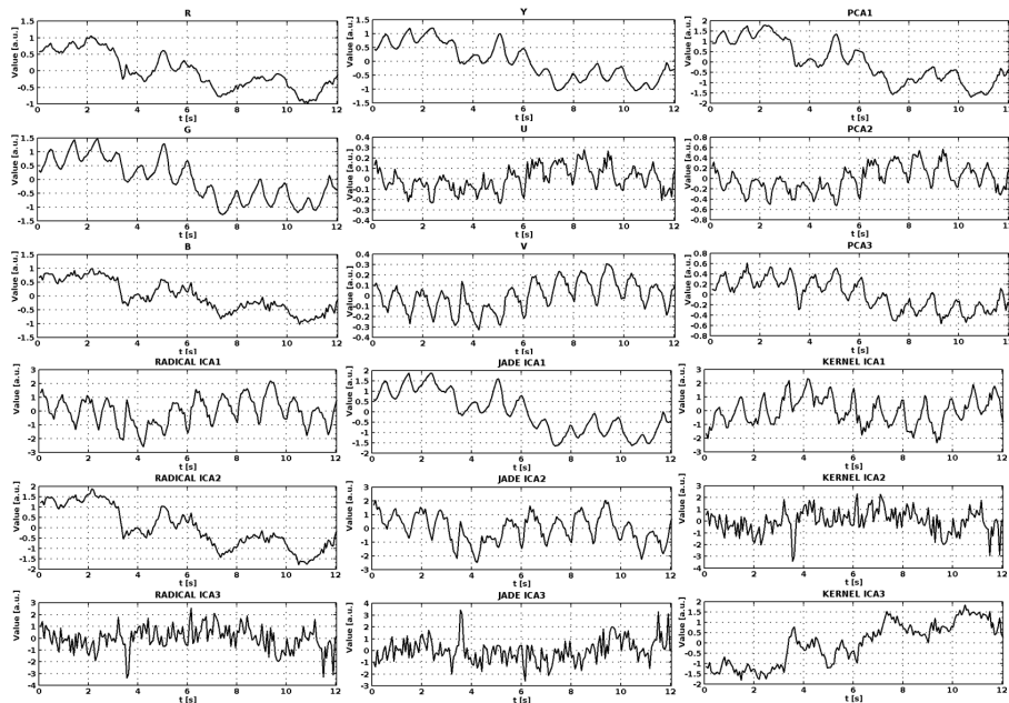
Fig. 2. An example of pre-processed signals obtained for: (top, left): a) RGB color model; b) YUV color model; c) PCA components from R , G , B signals; (bottom, left): RADICAL ICA, JADE ICA, KERNEL ICA.
