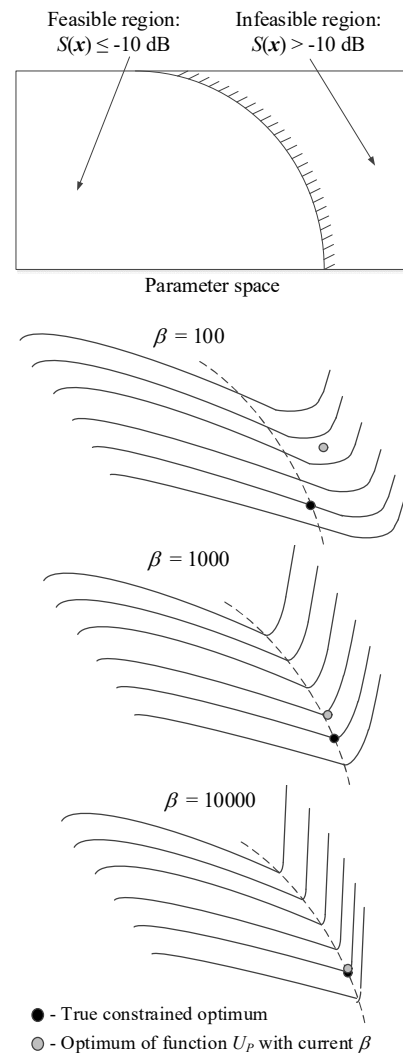
Fig. 1. Graphical illustration of the parameter space and feasible set using the example of antenna reflection constraint S(\mathbf{x}) \leq -10 dB with S(\mathbf{x}) = \max\{f \in F : |S_{11}(\mathbf{x}, f)|\} (cf. (5)): (a) feasible and infeasible sets, (b) landscapes of the objective function U_P (4) for the various values of the penalty coefficient \beta . The true optimum is located at the boundary of the feasible region. For small \beta , the objective function optimum is infeasible and may exhibit considerable constraint violation; for large values of \beta , the optimum approaches the true optimum; however, the optimization problem becomes numerically demanding due to very steep landscape in the vicinity of the feasible set boundary. The optimization result may become increasingly dependent on the initial design as traversing the boundary is hindered by the objective function nonlinearity.
