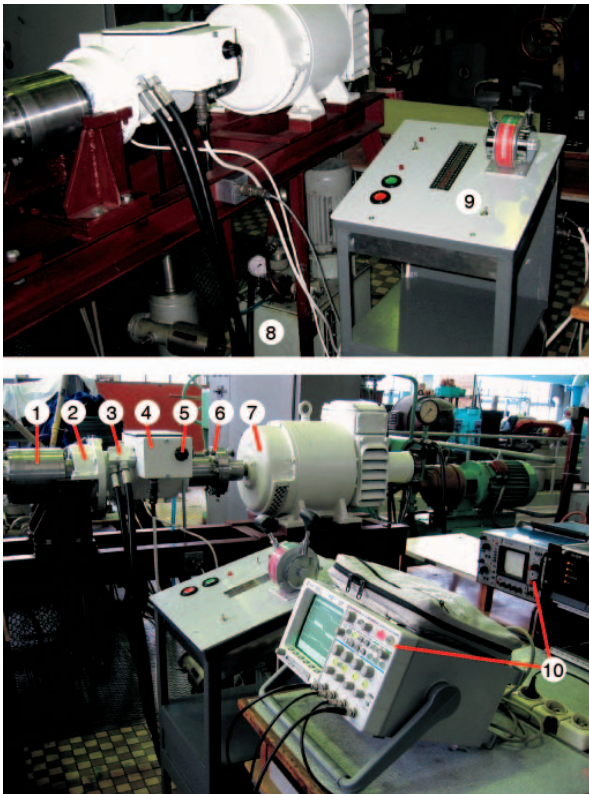
Fig. 3. The laboratory stand for testing the CP propeller servomechanism. Notation: 1 – hydraulic pitch control cylinder placed between flanges of propeller shaft and intermediate shaft; 2 – angular bearing; 3 – hydraulic distributor; 4 – oil timing box with internal control unit; 5 – hand wheel for propeller pitch local setting; 6 – clutch; 7 – shaft driving DC motor; 8 – hydraulic supply unit; 9 – remote control desk; 10 – measurement recording equipment
