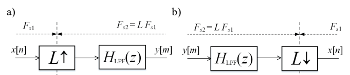
Fig. 1. Classic L -fold interpolator (a) and decimator (b).
