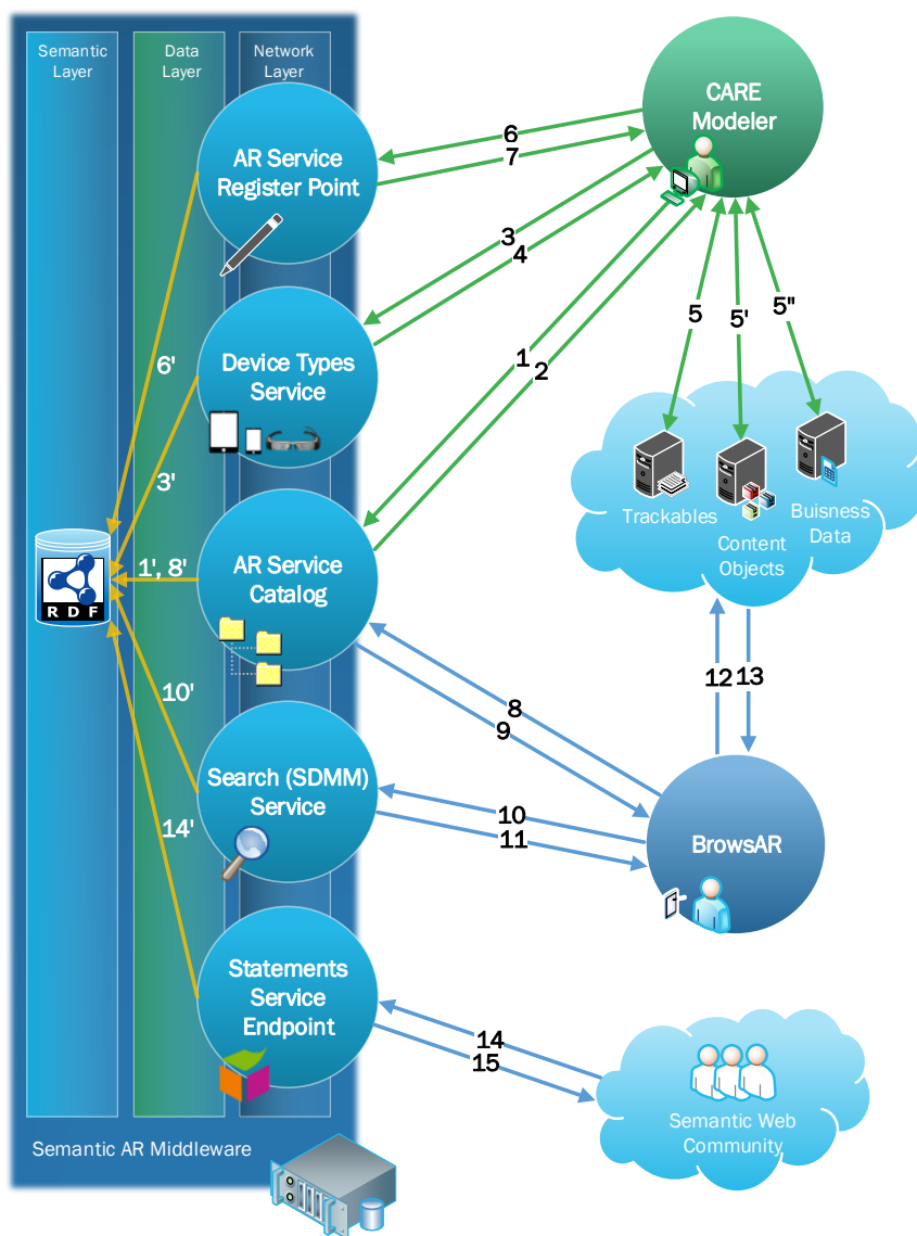
Figure 5.1: Data flow diagram of the CARE system.
