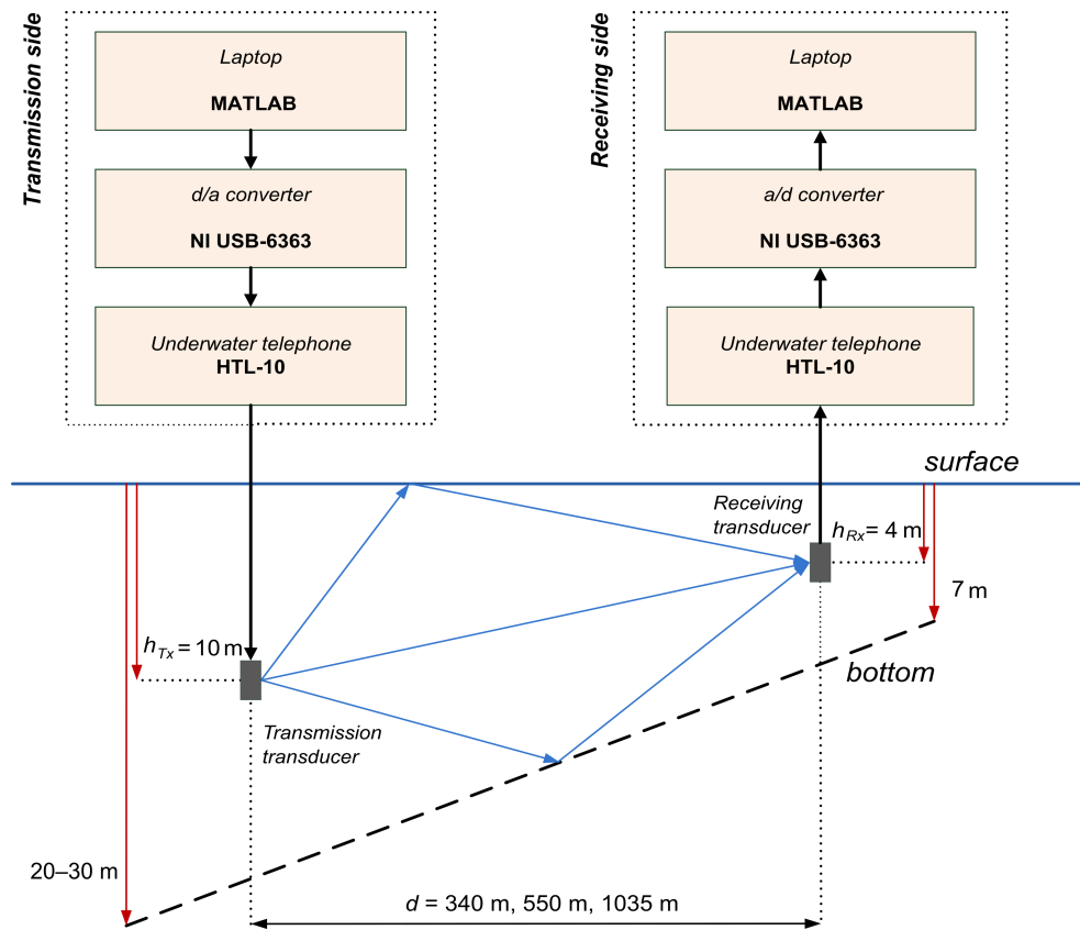
Fig. 3. Measuring system.
