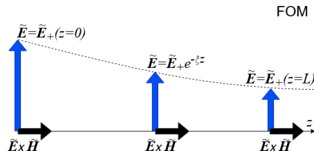
Figure 1. Considered plane wave propagating in medium described by FOM.
