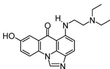
C-1311
