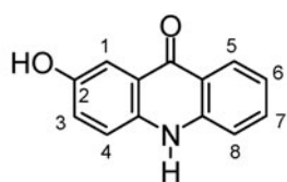
2-hydroxyacridinone
