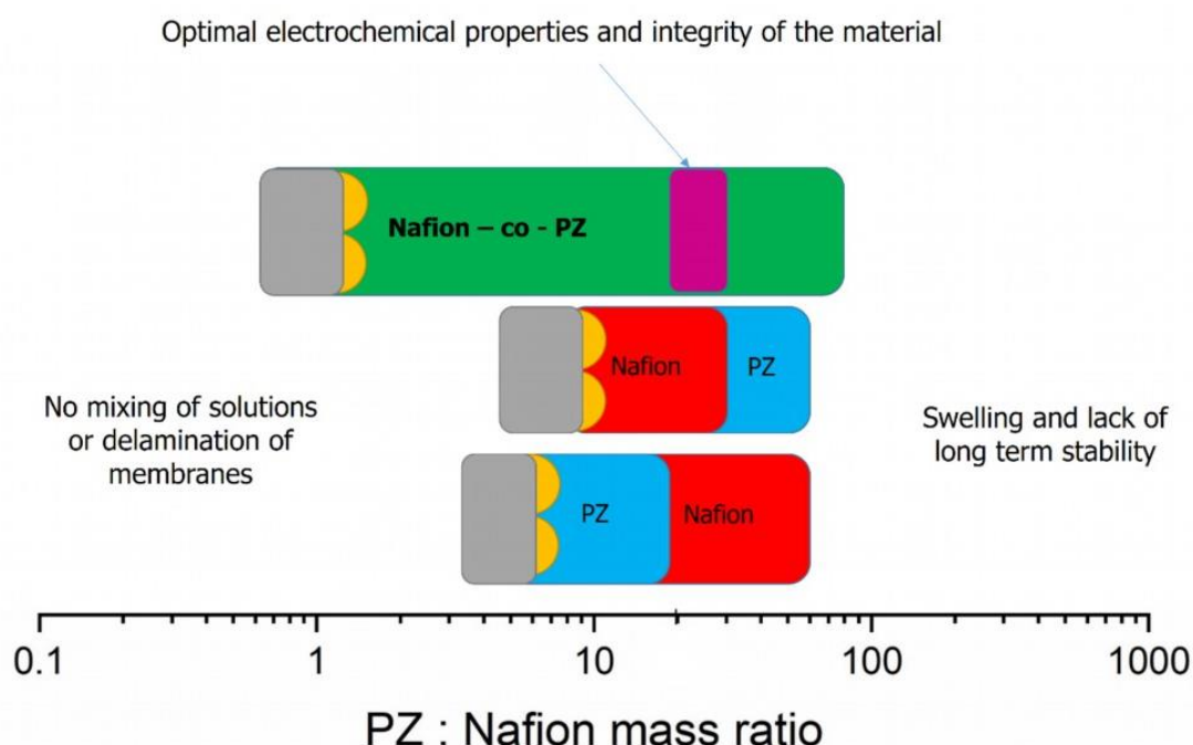
Fig. 5 Ranges of the integrity of the material for different hybrid coating configurations with respect to mass ratio of polymers.
