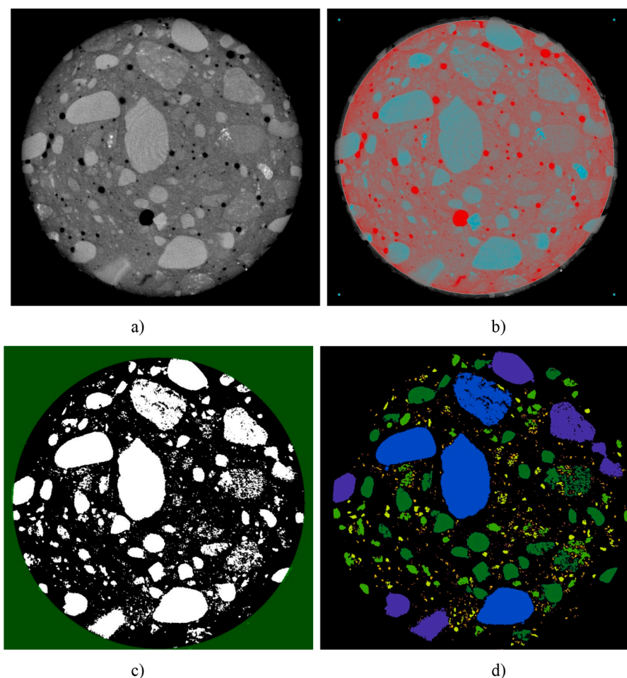
Fig. 2. Mid-section of specimen with diameter D = 74 mm: a) original scan image, b-d) region of interest (ROI) for further analyses [30].
