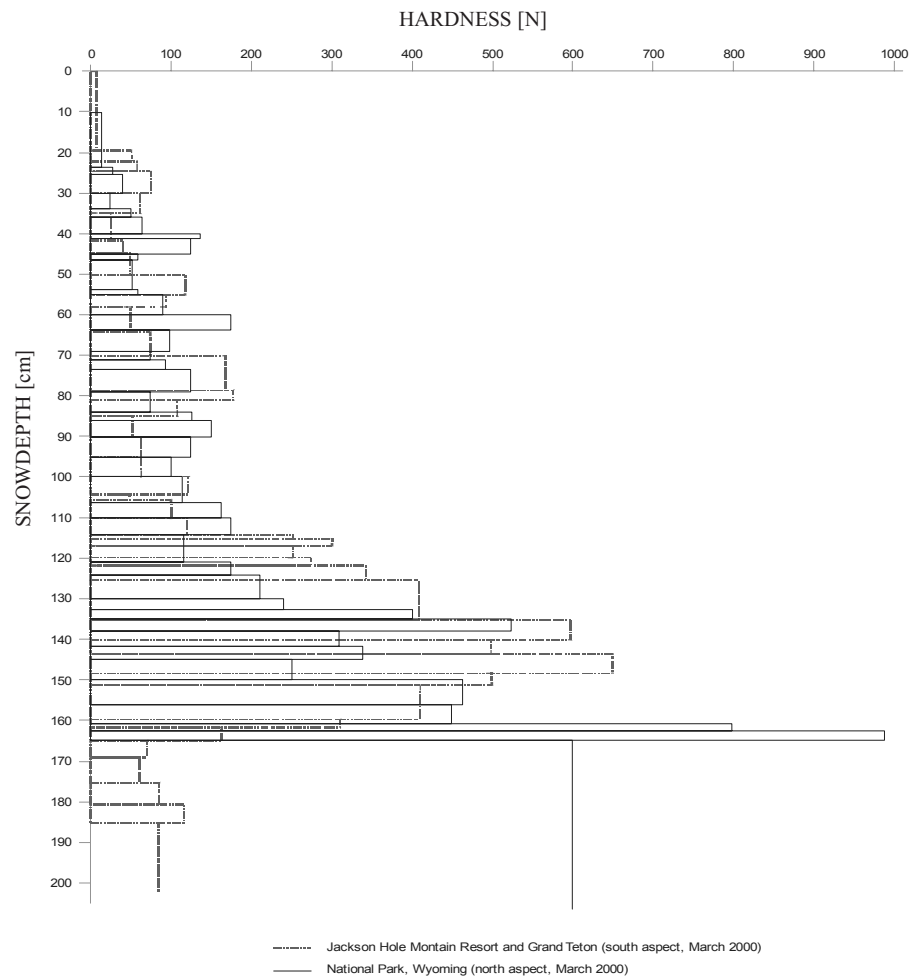
Fig. 4. Ram penetrometer profile of southern and northern aspects in March 2000 (Jackson Hole Mountain Resort and Grand Teton National Park, Wyoming) [24].
