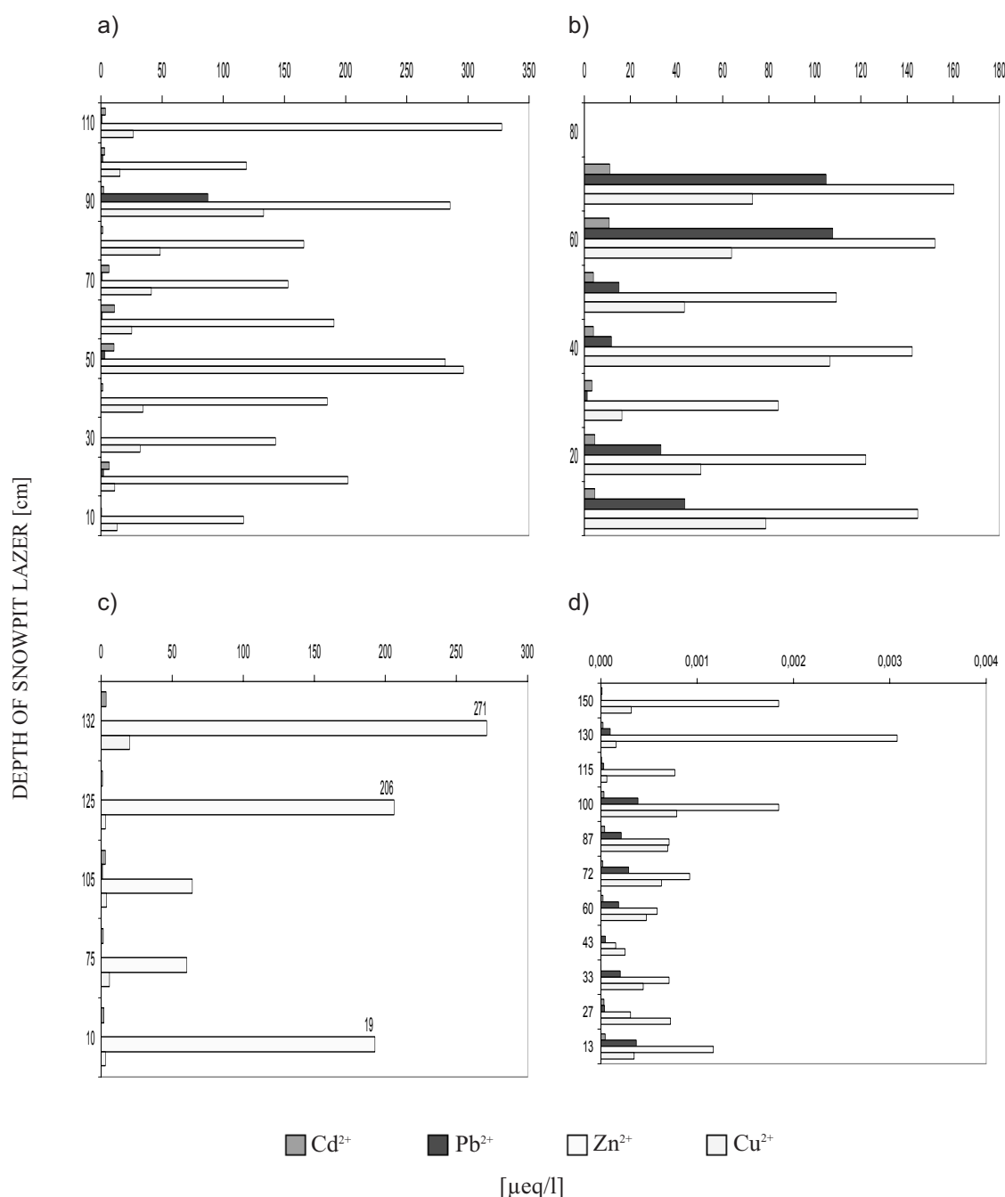
Fig. 11. Mean concentrations of cadmium, lead, zinc, and copper ions in snow samples collected at a) Śnieżnik, b) Orle, c) Szrenica in January 2008 (author's own results – concentrations of Zn 2+ and Cu 2+ x 10), d) the Greenland ice sheet (July 1992) [49].
