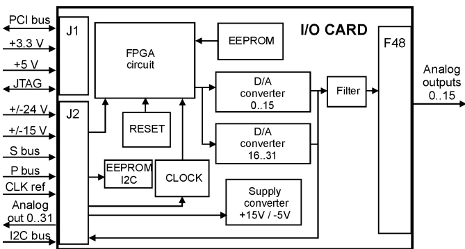
Fig. 5. I/O card block scheme.
