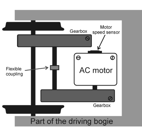
Fig. 2. Singular traction drive.
