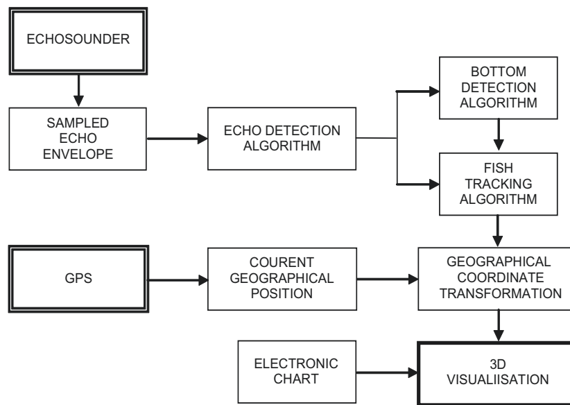
Fig. 7.4. Modern hydroacoustic fish data processing chain
