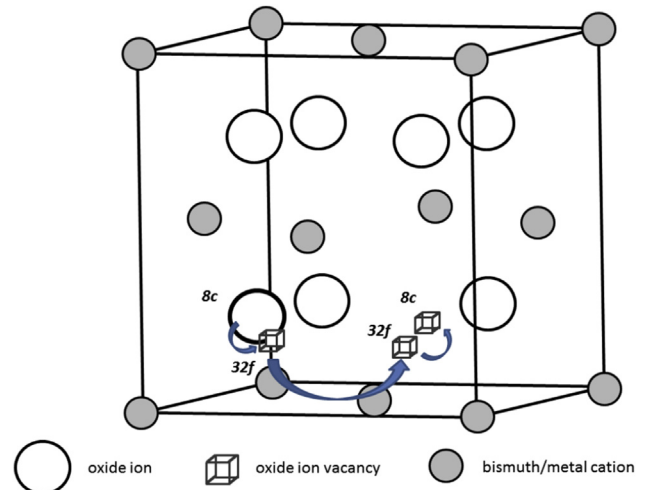
Fig. 6 – Scheme of oxide ion movements in the bismuth oxide based cubic fluorite type compounds.
