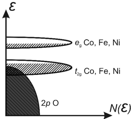
Fig. 13 – Schematic representation of the electronic structure of the \text{La}_{1-x}\text{Sr}_x\text{Co}_{1-y-z}\text{Fe}_y\text{Ni}_2\text{O}_{3-\delta} perovskites. Reprinted from Ref. [67], Copyright (2007), with permission from Elsevier.
