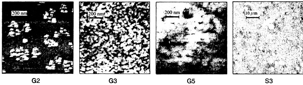
Fig. 2. AFM pictures of \text{Bi}_{0.33}\text{Ge}_{0.67}\text{O}_{1.84} (G2, G3 and G5) and \text{Bi}_{0.57}\text{Si}_{0.43}\text{O}_{1.72} (S3) glass samples.
