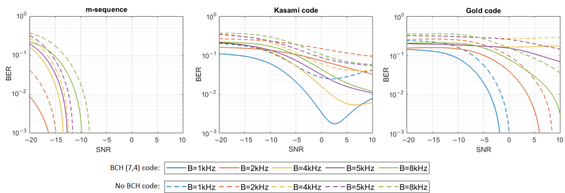
Figure 4. BER as a function of SNR for transmission in a UAC channel simulated using impulse response generated by 1 virtual source.
