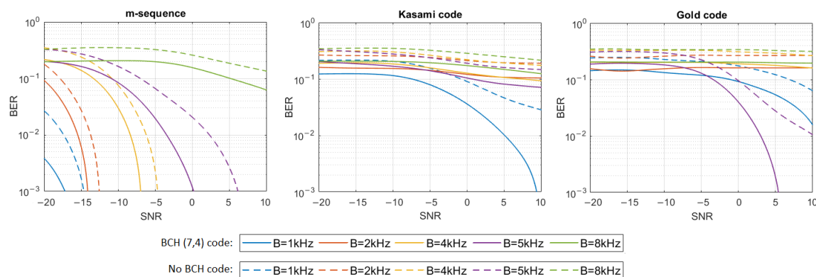
Figure 8. BER as a function of SNR for transmission in an UAC channel simulated using impulse response generated by 13 virtual sources.
