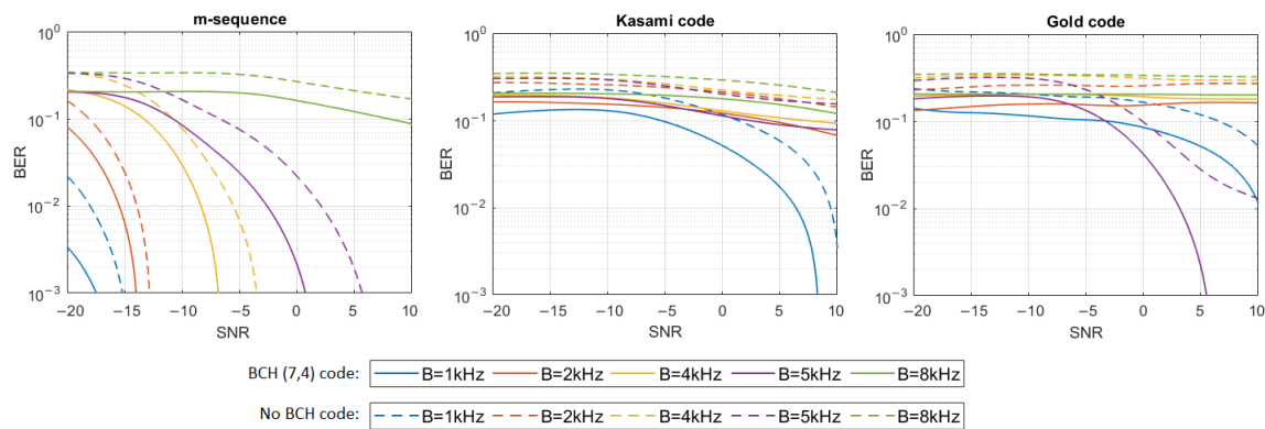
Figure 9. BER as a function of SNR for transmission in an UAC channel simulated using impulse response generated by 21 virtual sources.
