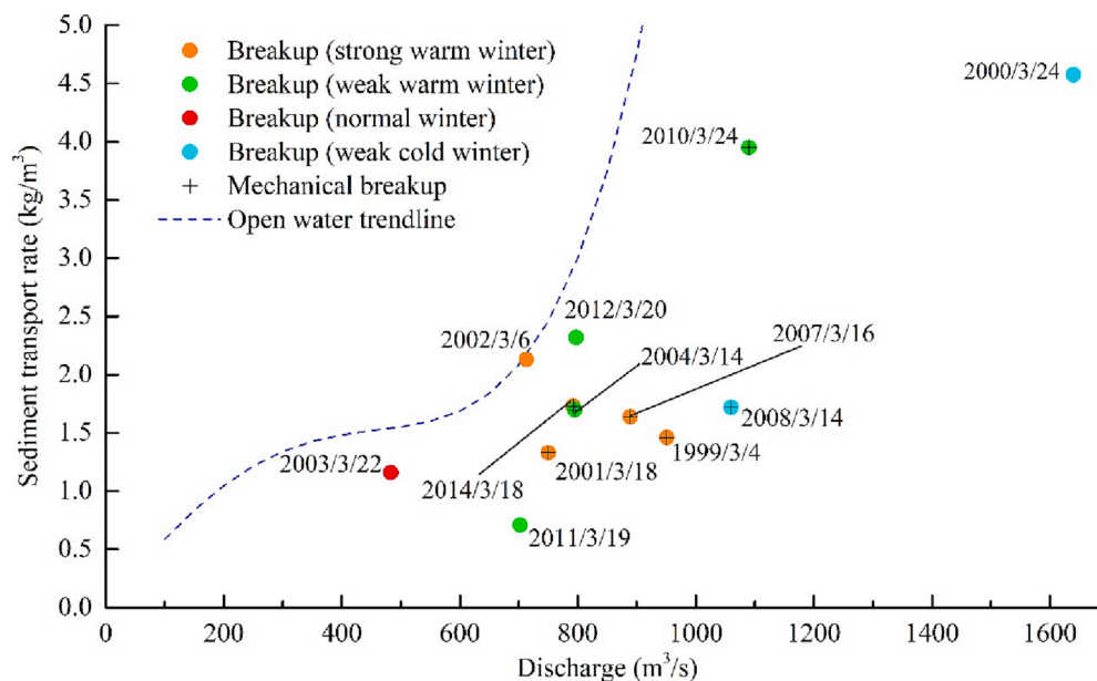
Fig. 11. Relationship between the suspended sediment transport rate and the discharge rate during breakup condition of different winter types (the breakup date).
