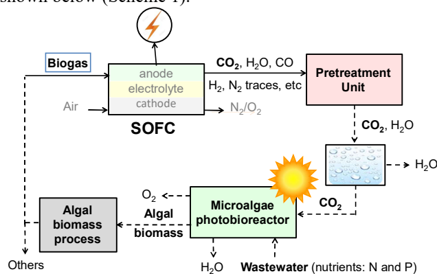
Scheme 1 Proposed system for cleaner and sustainable energy production. Included in this work (straight line), future research (dashed line)
