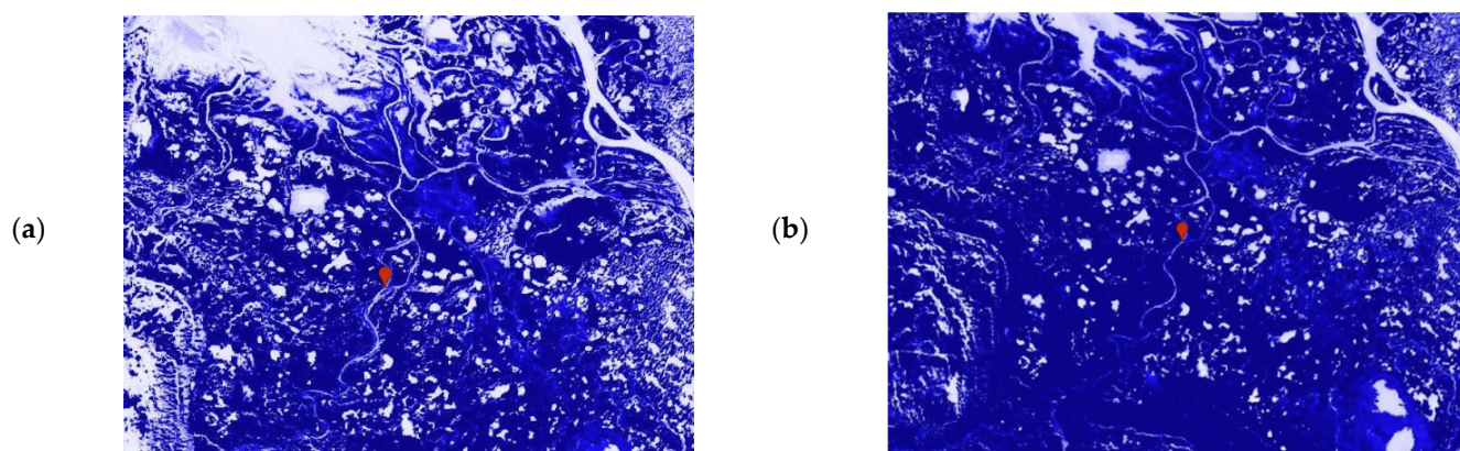
Figure 12. NDSII Results (a) for the image taken 14 May 2020, (b) for the image taken 13 June 2020.
