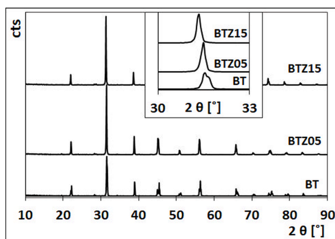
Fig. 1. XRD patterns of \text{BaTi}_{1-x}\text{Zr}_x\text{O}_3 ceramics at room temperature
