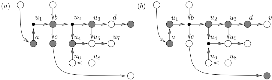
Fig. 5. (a) if the game started with c \rightarrow_W v , then W should not play u_5 \rightarrow_W u_7 ; (b) a configuration after 5 moves following d \rightarrow_W v .
