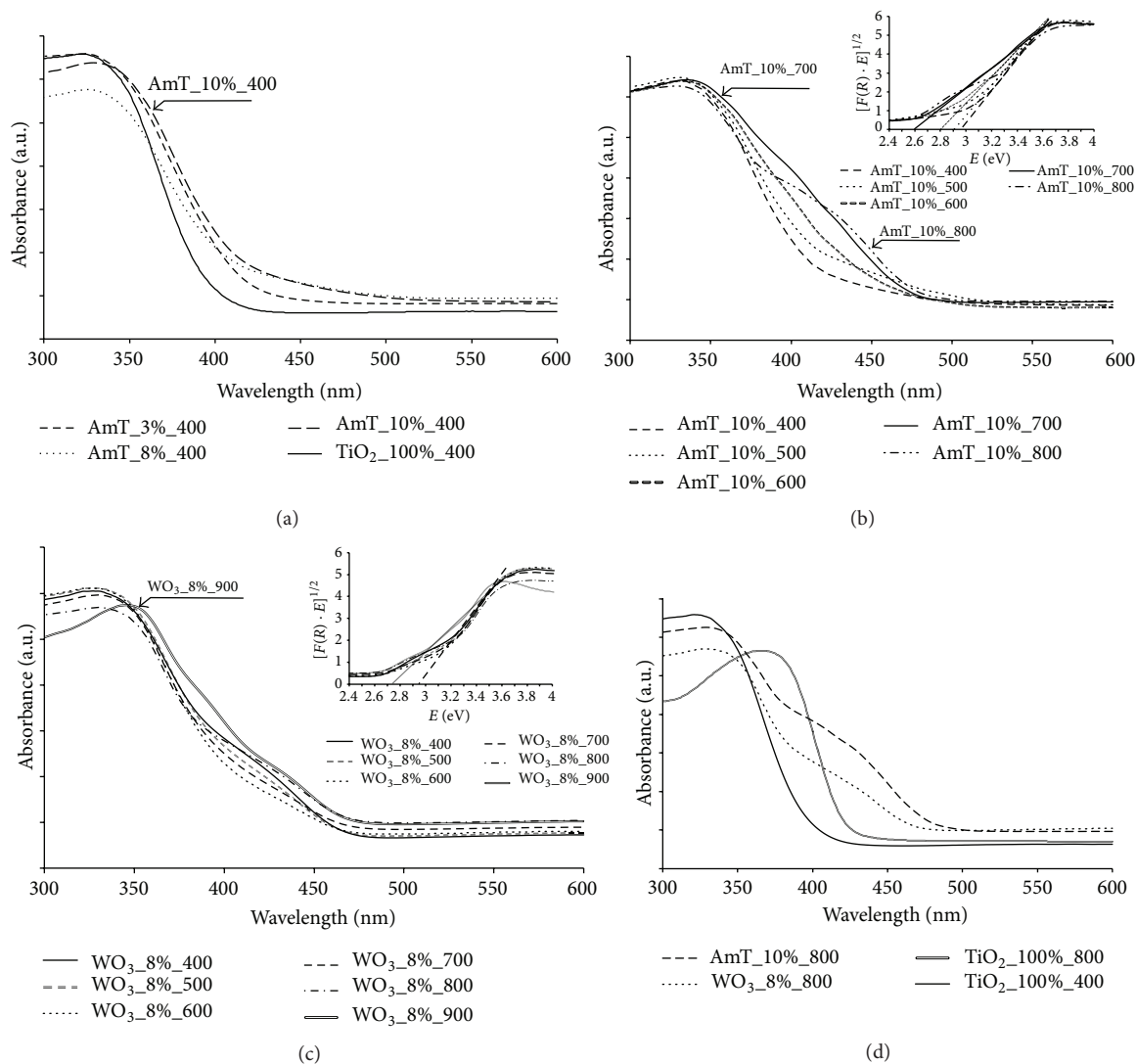
FIGURE 2: The DR/UV-Vis spectra of \text{WO}_3/\text{TiO}_2 with different amounts of ammonium metatungstate (a), \text{WO}_3/\text{TiO}_2 calcinated at 400, 500, 600, 700, and 800°C for \text{TiO}_2 modified with AmT (b), determination of indirect interband transition energies for \text{TiO}_2 modified with commercial \text{WO}_3 (c), and the DR/UV-Vis spectra of pure \text{TiO}_2 calcinated at 400°C and 800°C and \text{WO}_3/\text{TiO}_2 powders with the highest intensity of visible light absorption (d).
