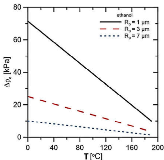
Figure 3. Capillary pressure rise characteristic for ethanol as a working fluid.
