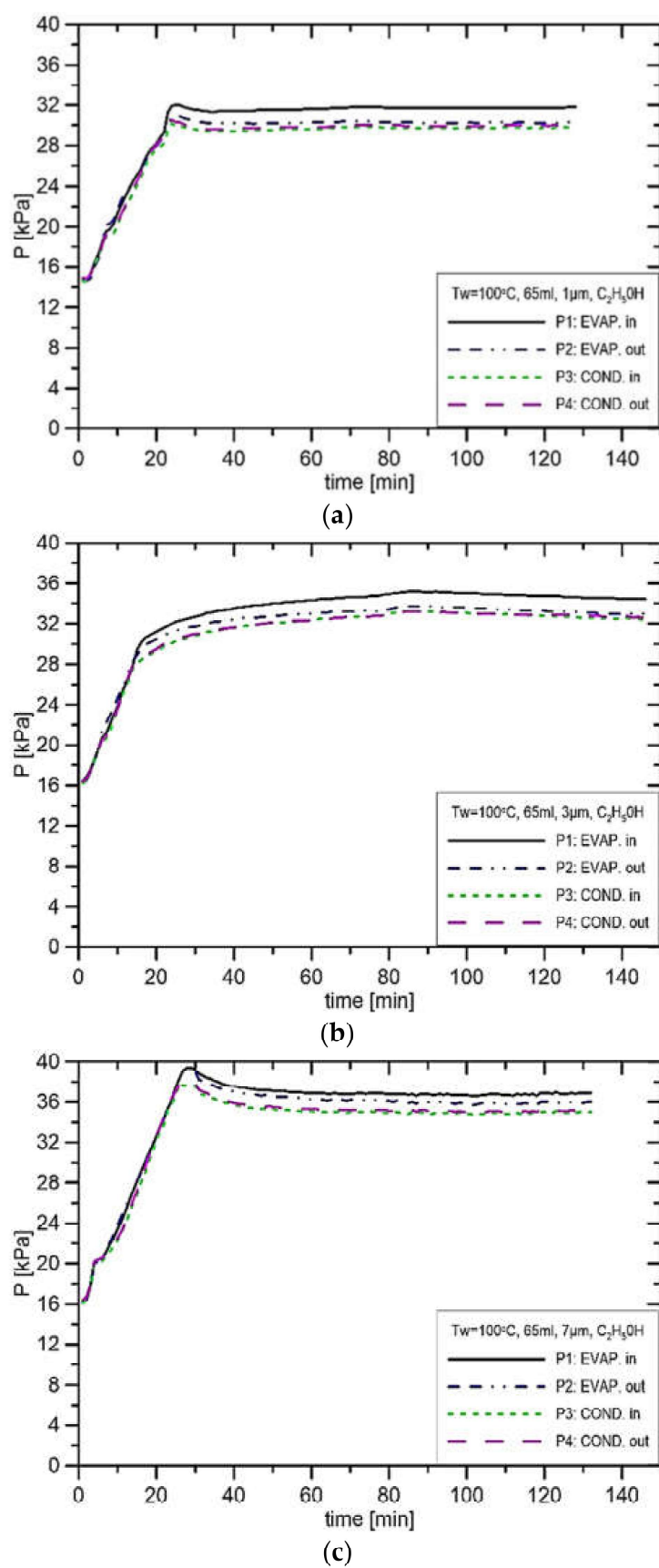
Figure 14. Distribution of pressure in function of time when using ethanol, charge volume 65 mL, T_w = 100^\circ\text{C} , (a) R_p = 1\ \mu\text{m} , (b) R_p = 3\ \mu\text{m} , (c) R_p = 7\ \mu\text{m} .
