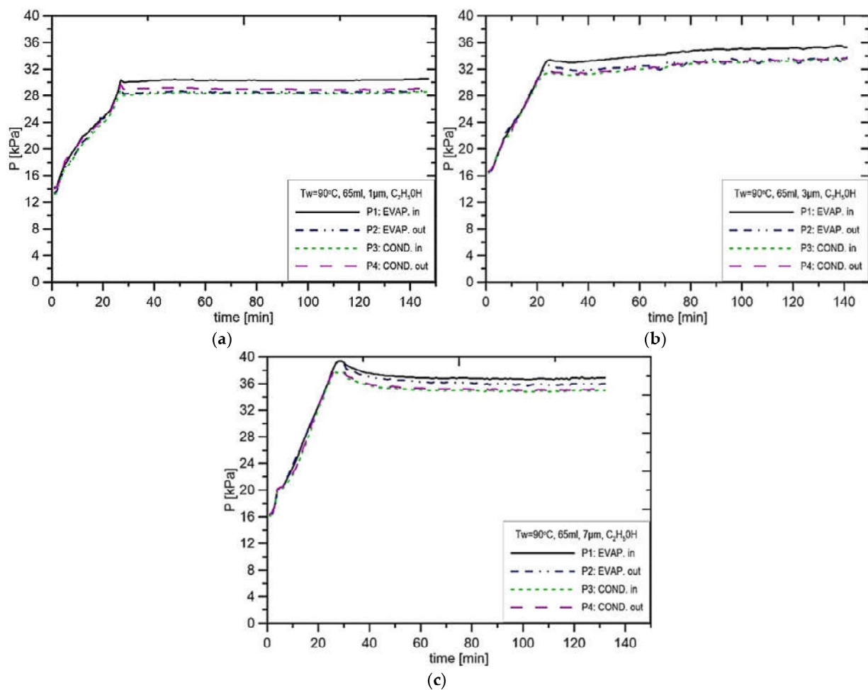
Figure 13. Distribution of pressure in function of time when using ethanol, charge volume 65 mL, T_w = 90^\circ\text{C} , (a) R = 1\ \mu\text{m} , (b) R_p = 3\ \mu\text{m} , (c) R_p = 7\ \mu\text{m} .
