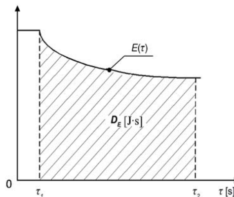
Fig. 4. Geometrical interpretation of the energy parameter characterising the potential of the energy source
