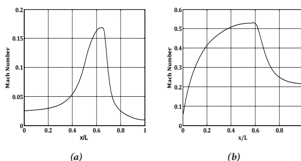
Fig. 8. Maximum air velocity for (a) An ellipse with \zeta = 3 and (b) An ellipse with \zeta = 7 .
