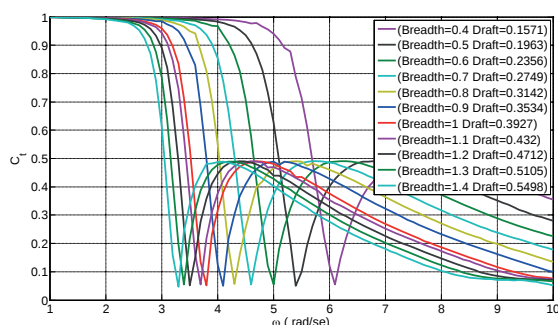
Fig. 20. C_t of rectangular pontoon section, type II
