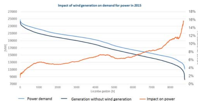
Fig. 6. Impact of wind generation on power demand in 2015. Own study based on data from [5]
