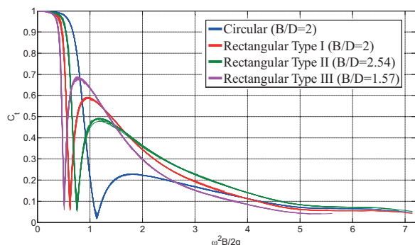
Fig. 25. C_t comparison of circular section and three similar rectangular sections versus normalized frequency
