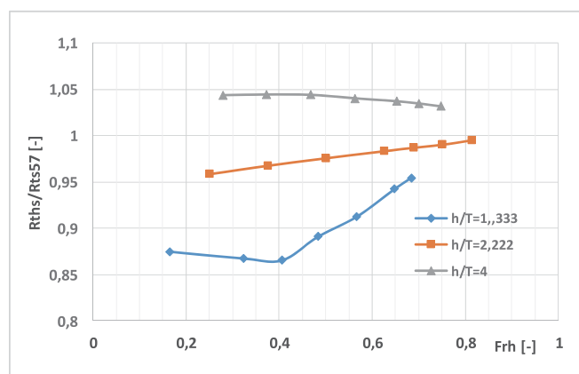
Fig.10. The effect of water depth, 2 \times T170 at T = 0.90 m
