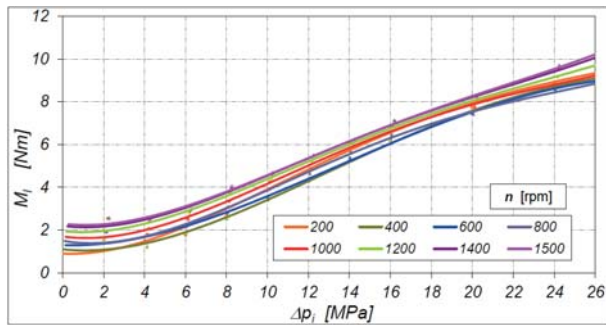
Fig. 10. Characteristics of M_l = f(\Delta p_i) . Working medium: oil
