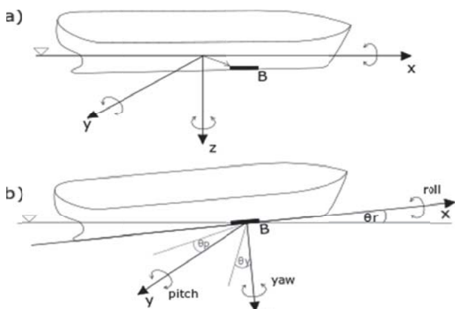
Fig. 10. Ship motions caused by sea surface waving
