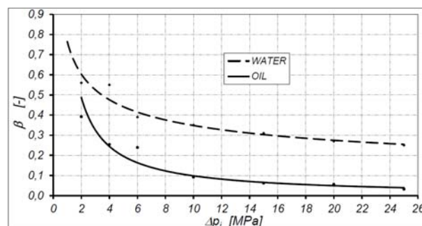
Fig. 18. Characteristics of \beta = f(\Delta p_i) . Working medium: oil and water
