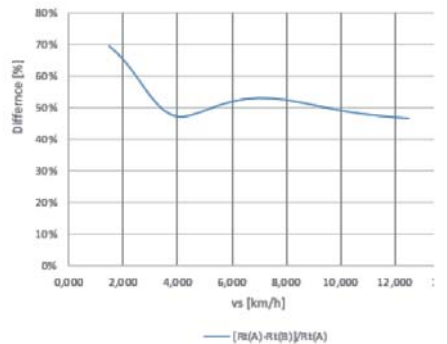
Fig. 14 Increase in the resistance [ % ]
