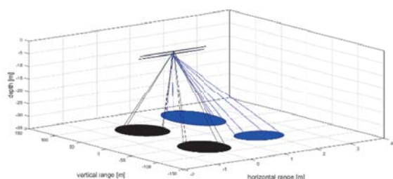
Fig. 17. Footprint of the side scan sonar \theta_r = 5^\circ, \theta_p = 3^\circ
