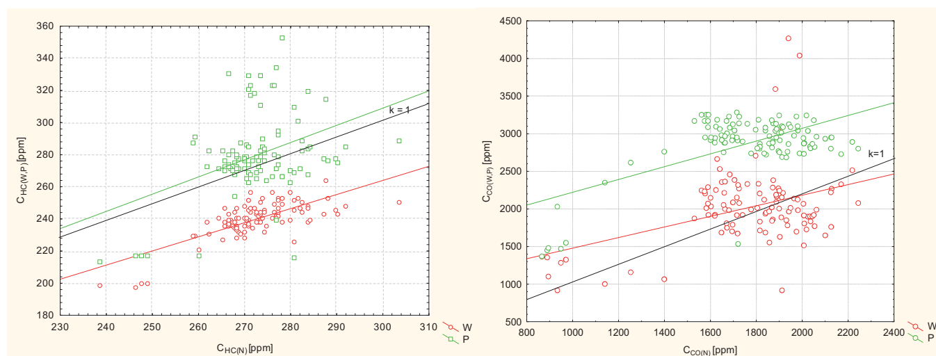
Fig. 6. Values of HC and CO concentration for transient state at n = 1100 rpm and load change from T_q = 0 Nm to T_q = 70 Nm: C_{HC(N, W, P)} – HC concentration, C_{CO(N, W, P)} – CO concentration for nominal (N), advanced (W), and delayed (P) fuel injection timing
