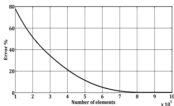
Fig. 9. Mesh dependency analysis
