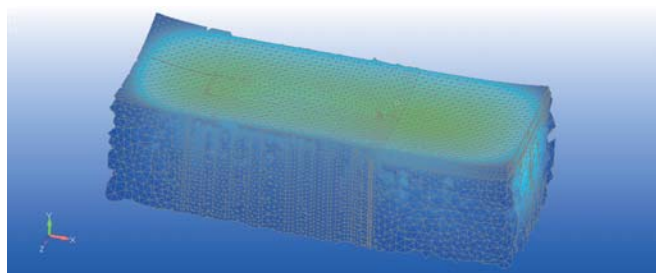
Fig. 9. Deformed mesh of finite elements of water mass around moving ship
