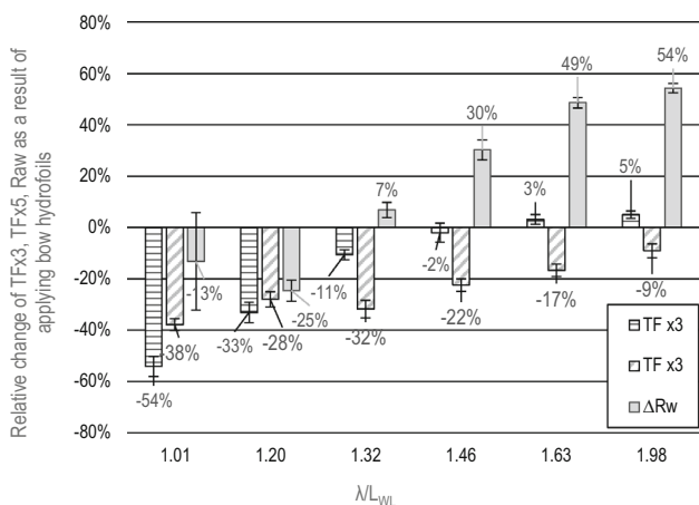
Fig. 24 Effect of adding bow hydrofoils ( AoA = 0 deg) on heave (TF \times 3 ), pitch (TF \times 5 ), and added resistance (raw)
