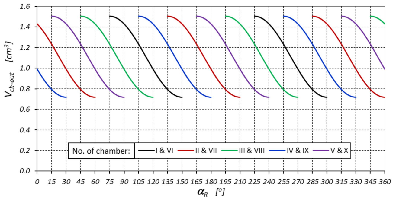
Fig. 8. Characteristics of the volume V_{ch-out} of the chambers with decreasing volume (emptied) as a function of the angle of rotation \alpha_R of the rotor (within one complete rotation of the rotor – \alpha_R = 360^\circ ).
