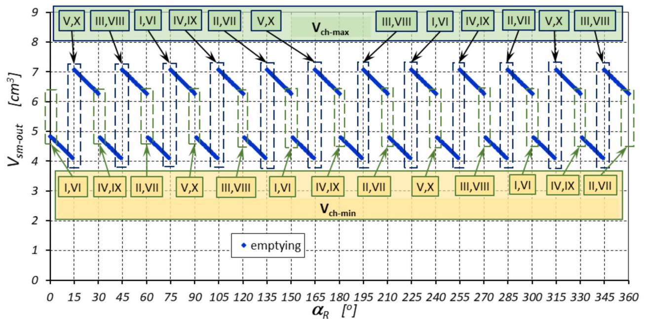
Fig. 10. Volume V_{sm-out} of the emptied working chambers as a function of the angle of rotation \alpha_R of the rotor (within one complete rotation of the rotor – \alpha_R = 360^\circ ).
