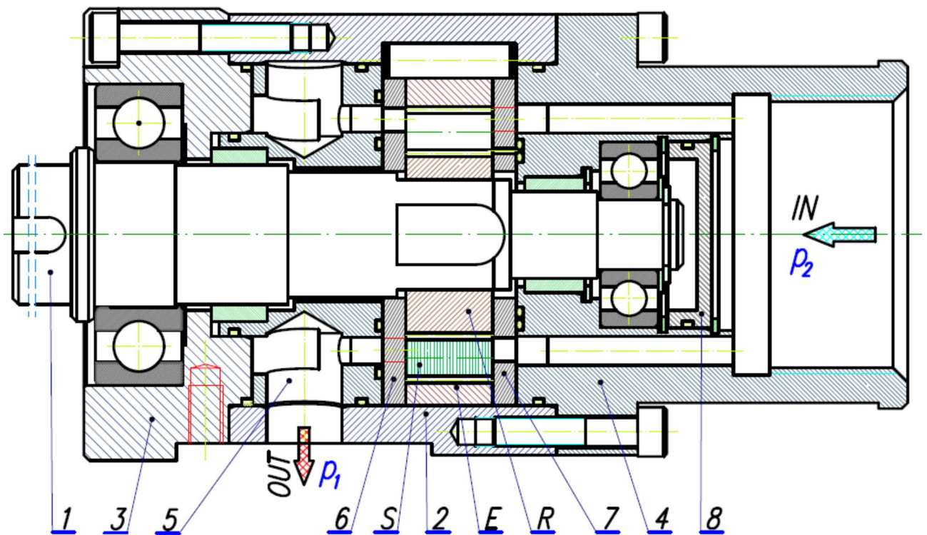
Fig. 25. Tested pump (satellite pump): E – external gear (curvature), S – satellite, R – rotor, 1 – shaft, 2 and 3 – housing, 4 – suction (inflow) manifold, 5 – pumping (outflow) manifold, 6 – high-pressure commutation (compensation) plate, and 7 – low-pressure commutation (compensation) plate, 8 – cover of the shaft chamber.
