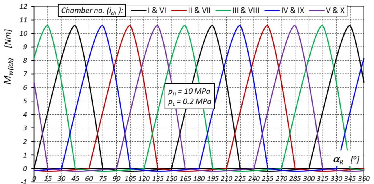
Fig. 21. Characteristics of the torque M_{w(ich)} “generated” by all working chambers as a function of the angle of rotation \alpha_R of the rotor (within one complete rotation of the rotor – \alpha_R=360^\circ ).
