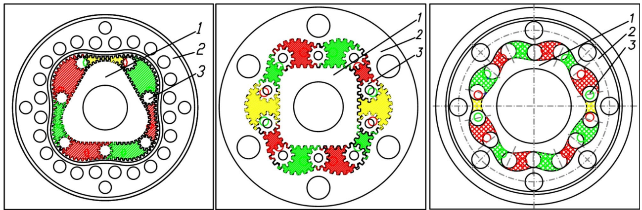
Fig. 1. Satellite mechanisms: type 3 \times 4 (left), type 4 \times 6 (middle) and type 6 \times 8 (right): 1—rotor, 2—curvature, 3—satellite 15 .
