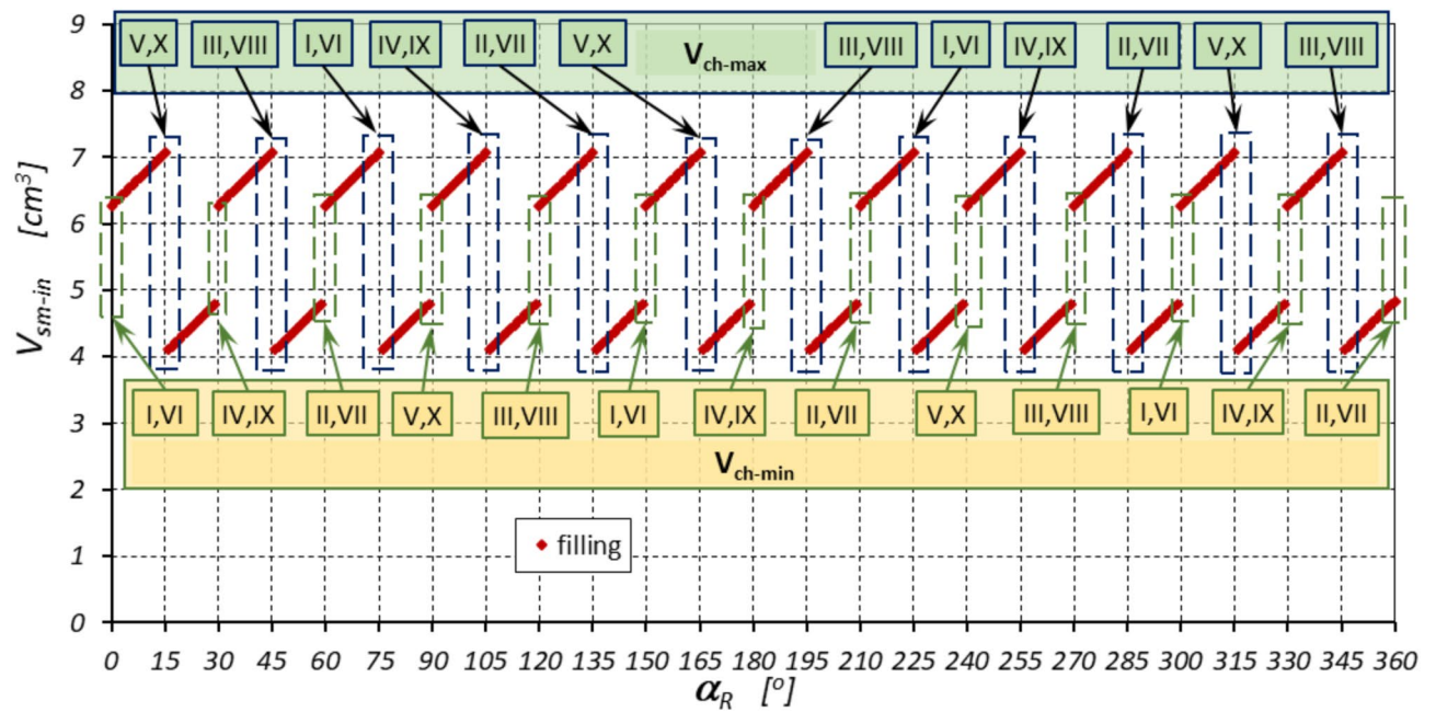
Fig. 9. Volume V_{sm-in} of the filled working chambers as a function of the angle of rotation \alpha_R of the rotor (within one complete rotation of the rotor – \alpha_R = 360^\circ ).
