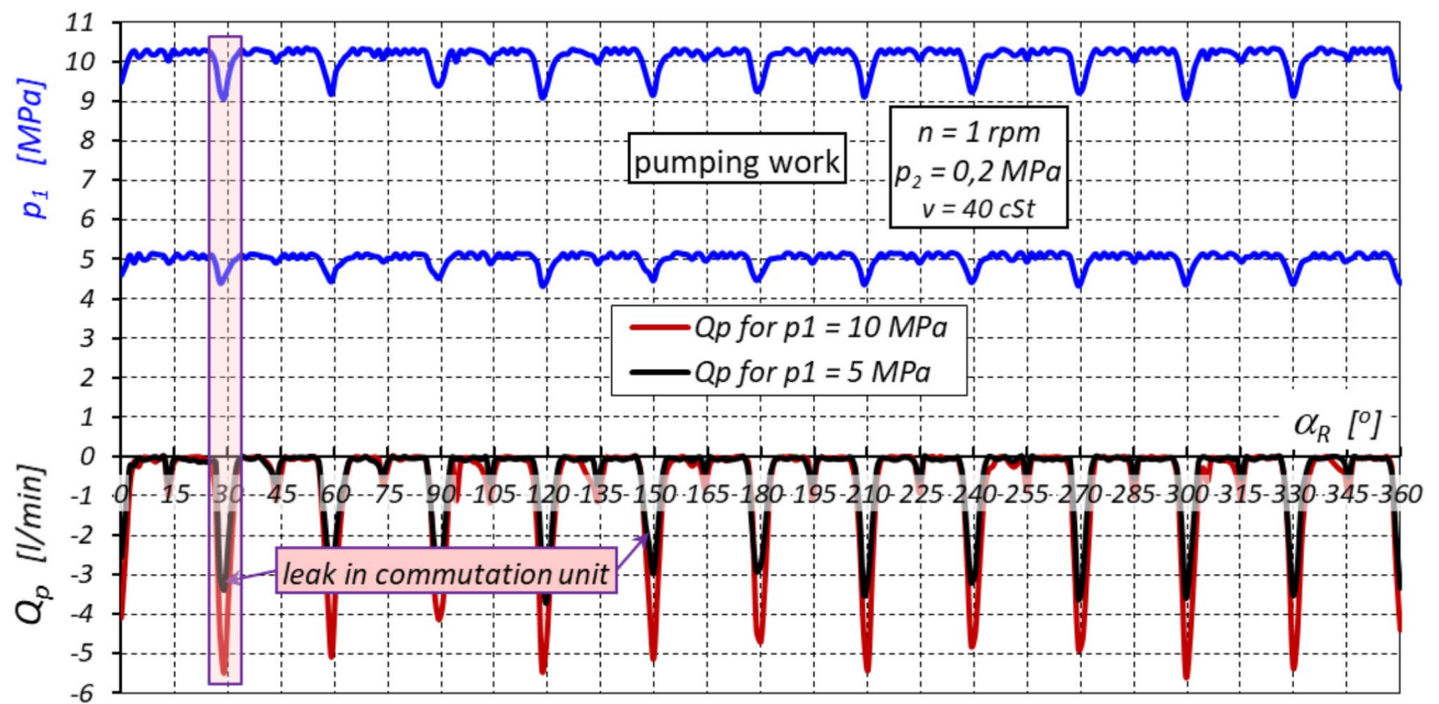
Fig. 30. Characteristics of the actual flow rate Q_p in the machine working as a pump as a function of the angle of rotation \alpha_R of the rotor (within one complete rotation of the rotor – \alpha_R = 360^\circ ). The pressure loading the pump: p_1 = 5 MPa and p_1 = 10 MPa.
