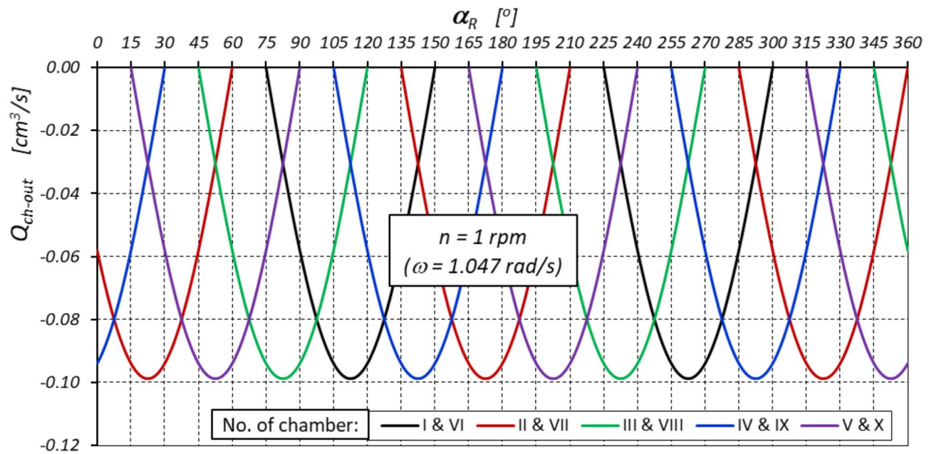
Fig. 13. Characteristics of the liquid flow rate Q_{ch-out} in the emptied chambers as a function of the angle of rotation \alpha_R of the rotor (within one complete rotation of the rotor – \alpha_R = 360^\circ ).
