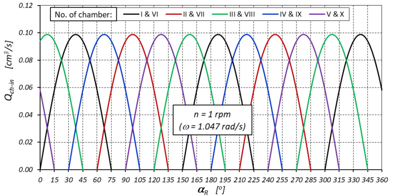
Fig. 12. Characteristics of the liquid flow rate Q_{ch-in} in the filled chambers as a function of the angle of rotation \alpha_R of the rotor (within one complete rotation of the rotor – \alpha_R = 360^\circ ).
