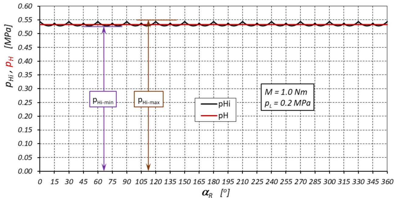
Fig. 24. Characteristics of the instantaneous p_{Hi} and the average pressure p_H as a function of the angle of rotation \alpha_R of the rotor (within one complete rotation of the rotor – \alpha_R = 360^\circ ).
