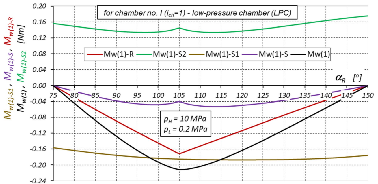
Fig. 19. Characteristics of the torque “generated” by working chamber No. I ( i_{ch}=1 ) in the range of the shaft rotation angle \alpha_R , which corresponds to the change in chamber volume from V_{ch-max} to V_{ch-min} (low pressure p_L in the chamber).
