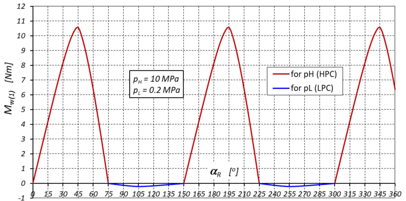
Fig. 20. Characteristics of the torque “generated” by the working chamber No. I ( i_{ch}=1 ) as a function of the angle of rotation \alpha_R of the rotor (within one complete rotation of the rotor – \alpha_R=360^\circ ).
