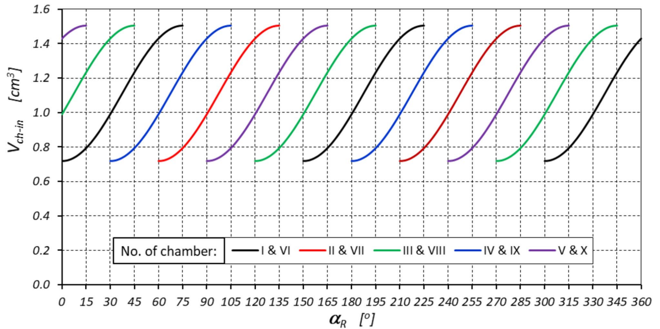
Fig. 7. Characteristics of the volume V_{ch-in} of the chambers with increasing volume (filled) as a function of the angle of rotation \alpha_R of the rotor (within one complete rotation of the rotor – \alpha_R = 360^\circ ).
