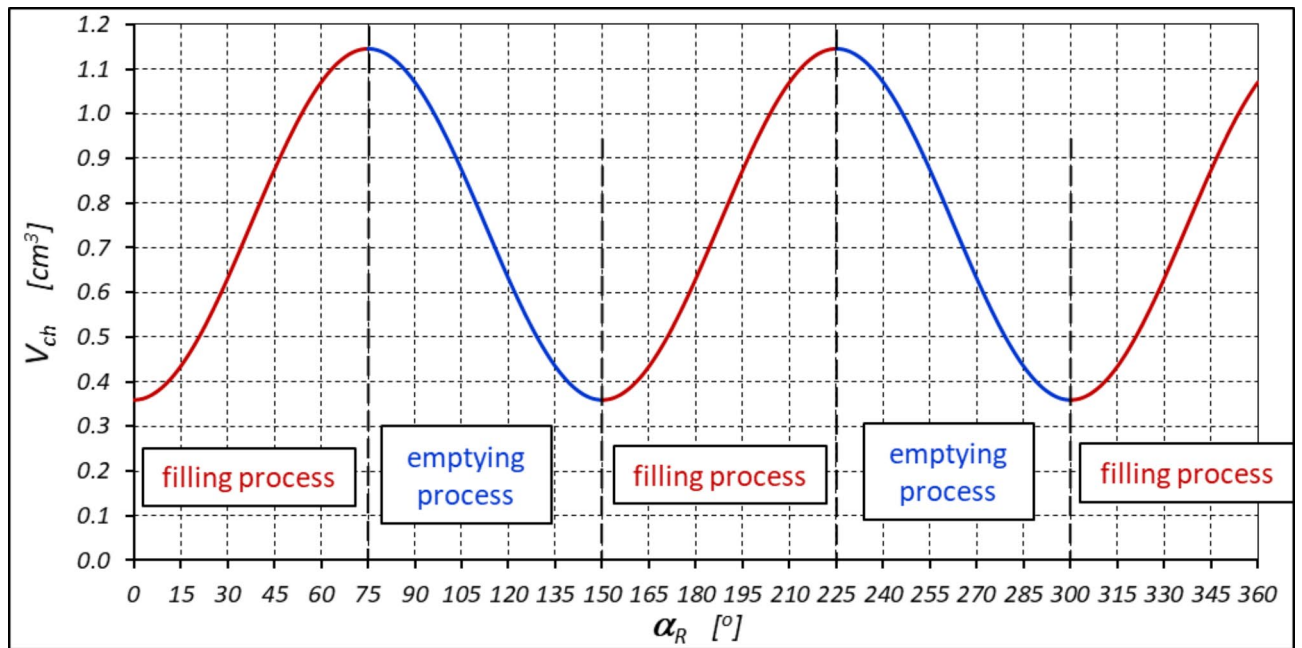
Fig. 5. The volume V_{ch} of the working chamber of the satellite mechanism as a function of the angle of rotation \alpha_R of the rotor (within one complete rotation of the rotor – \alpha_R = 360^\circ ).
