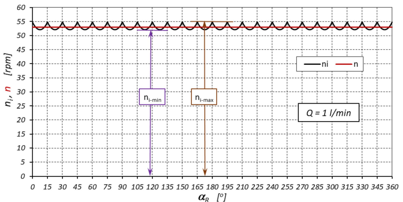
Fig. 16. Characteristics of instantaneous rotational speed n_i and the average rotational speed n of the rotor (shaft) as a function of the angle of rotation \alpha_R of the rotor (within one complete rotation of the rotor – \alpha_R = 360^\circ ).
