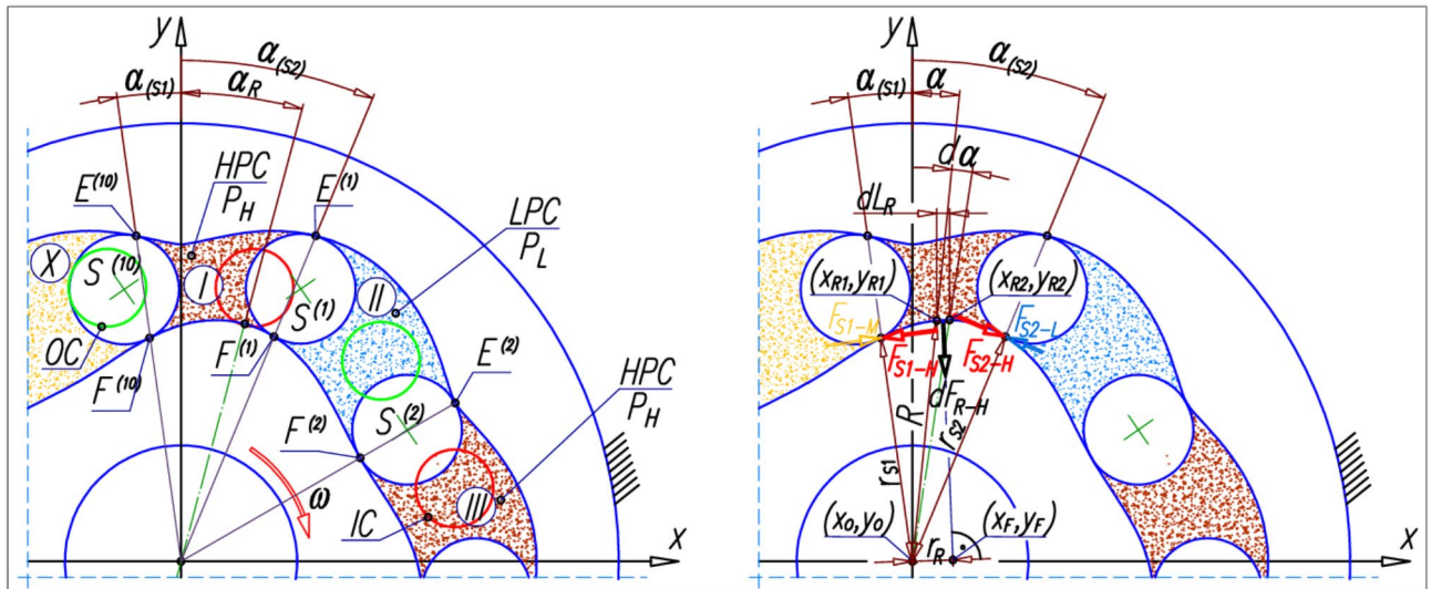
Fig. 17. The basic parameters of the satellite mechanism for calculating the torque. Description in the text. (created in Autodesk Autocad 2024, https://www.autodesk.com/ )
