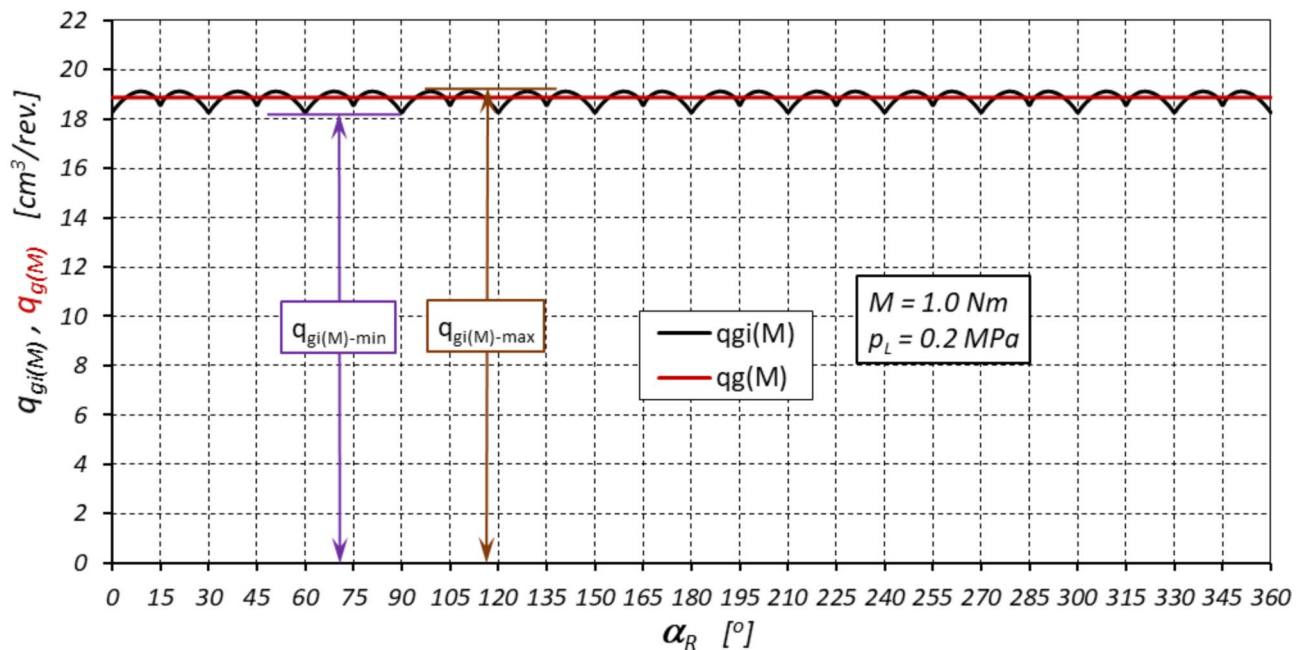
Fig. 23. Characteristics of the instantaneous torque working volume q_{gi(M)} and the average torque working volume q_g(M) as a function of the angle of rotation \alpha_R of the rotor (within one complete rotation of the rotor – \alpha_R = 360^\circ ).
