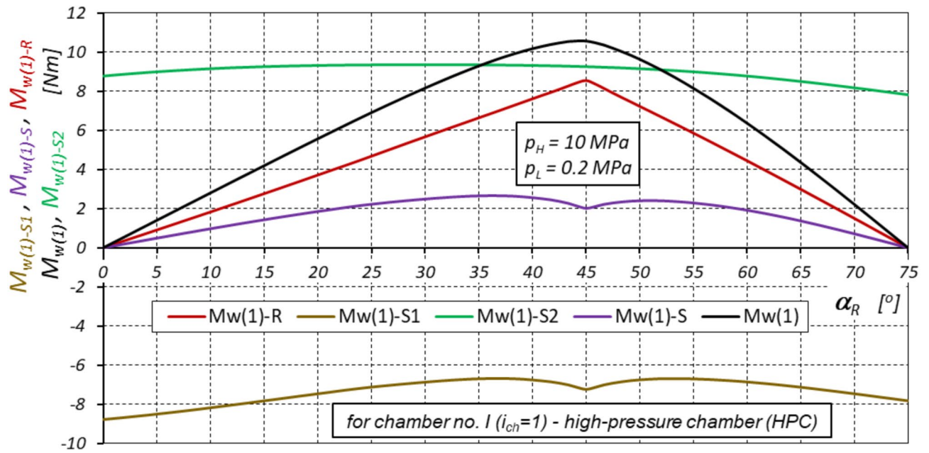
Fig. 18. Characteristics of the torque “generated” by working chamber No. I ( i_{ch}=1 ) in the range of the shaft rotation angle \alpha_R , which corresponds to the change in chamber volume from V_{ch-min} to V_{ch-max} (high pressure p_H in the chamber).
