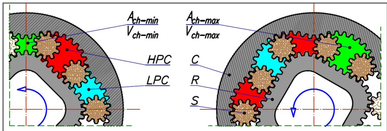
Fig. 2. Satellite mechanism type 4 × 6: C – curvature, R – rotor, S – satellite, HPC – high-pressure working chamber, LPC – low-pressure working chamber, A_{ch-min} – area of the chamber with minimum volume V_{ch-min} , A_{ch-max} – area of the chamber with maximum volume V_{ch-max} 34,44 .
