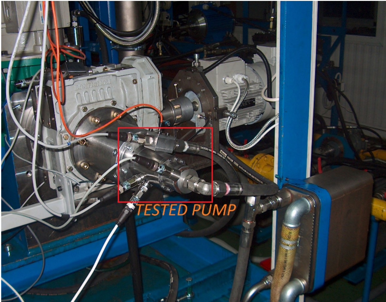
Fig. 29. View of the test stand with worm gear (grey colour) (left) and the satellite pump on the test stand (right).
