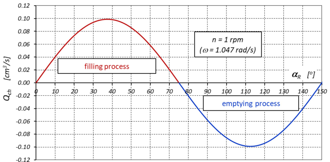
Fig. 11. Characteristics of the flow rate Q_{ch} in the one working chamber as a function of the angle of rotation \alpha_R of the rotor (shaft).
