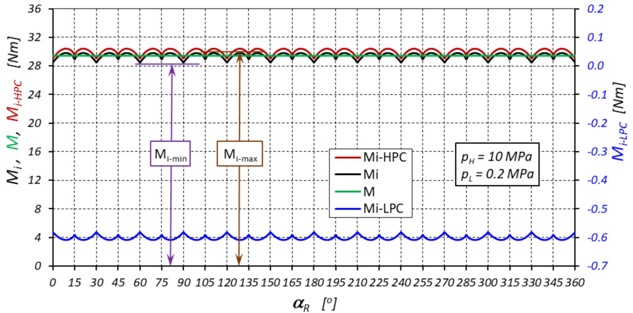
Fig. 22. Characteristics of the torque “generated” by the low-pressure working chambers ( M_{i-LPC} ) and the high-pressure working chambers ( M_{i-HPC} ). Characteristics of the instantaneous torque M_i and the average torque M as a function of the angle of rotation \alpha_R of the rotor (within one complete rotation of the rotor – \alpha_R = 360^\circ ).
