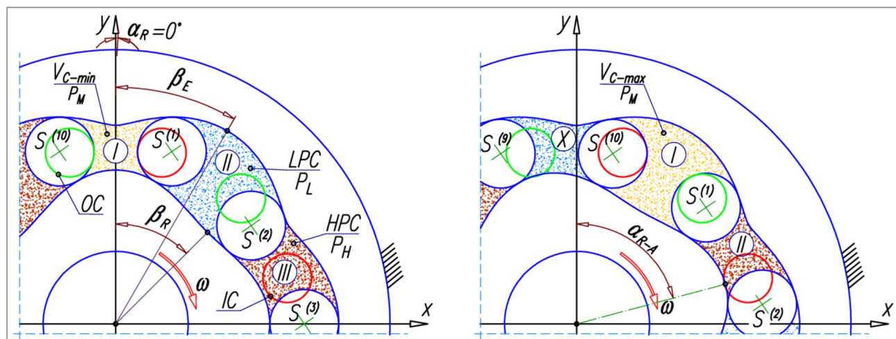
Fig. 3. Satellite mechanism type 4 × 6: \beta_R and \beta_E – characteristics angle of the rotor R and curvature (description in the text), S^{(1)} \div S^{(10)} – satellites, IC – inflow channel, OC – outflow channel, p_H – high pressure, p_L – low pressure, p_M – medium pressure, \alpha_R – angle of the rotor (shaft) rotation, \alpha_{R-A} – angle of rotor rotation for change from V_{min} to V_{max} , \omega – angular velocity of the rotor, I ÷ X – working chambers. (created in Autodesk Autocad 2024, https://www.autodesk.com/ )
