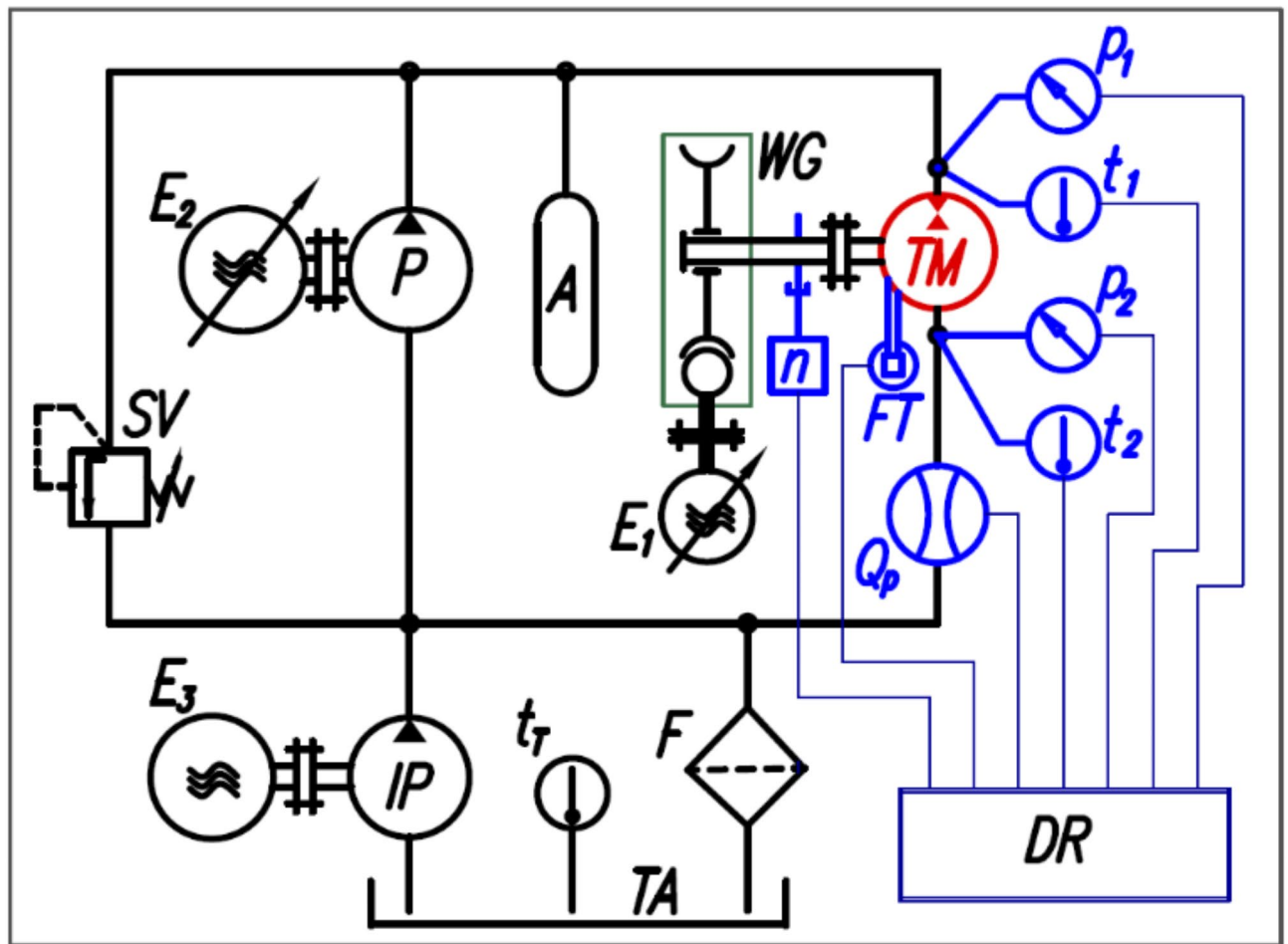
Fig. 28. The test stand – hydraulic system and measuring system: P – pump, TM – tested machine (pump or motor), IP – impeller pump (centrifugal pump), SV – safety valve, F – filter, TA – tank, WG – self-locking worm gear, E 1 and E 2 – electric motors with frequency converters, E 3 – electric motor, DR – data recorder, p 1 , p 2 – pressure transducers, t 1 , t 2 , t T – temperature transducers, Q p – flowmeter, FT – force transducer for torque M measurement, n – inductive sensor for rotational speed measurement. (created in Autodesk Autocad 2024, https://www.autodesk.com/ )
