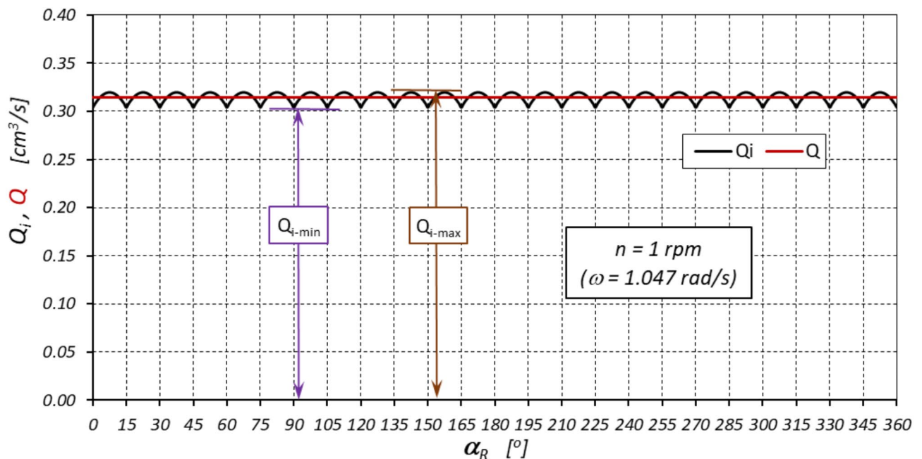
Fig. 14. Characteristics of instantaneous flow rate Q_i and average flow rate Q in the satellite mechanism as a function of the angle of rotation \alpha_R of the rotor (within one complete rotation of the rotor – \alpha_R = 360^\circ ).
