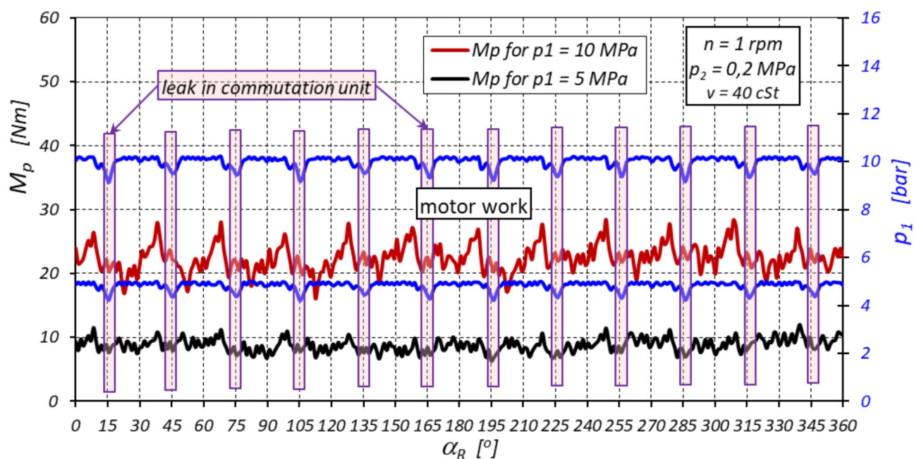
Fig. 33. Characteristics of the torque M_p on the shaft of the machine working as a motor as a function of the angle of rotation \alpha_R of the rotor (within one complete rotation of the rotor – \alpha_R = 360^\circ ). The pressure in the inflow port of the motor: p_1 = 5 MPa and p_1 = 10 MPa.
