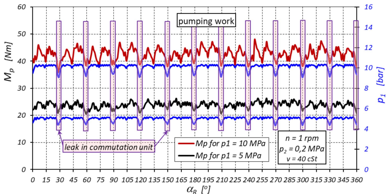
Fig. 32. Characteristics of the torque M_p on the shaft of the machine working as a pump as a function of the angle of rotation \alpha_R of the rotor (within one complete rotation of the rotor – \alpha_R = 360^\circ ). The pressure loading the pump: p_1 = 5 MPa and p_1 = 10 MPa.
