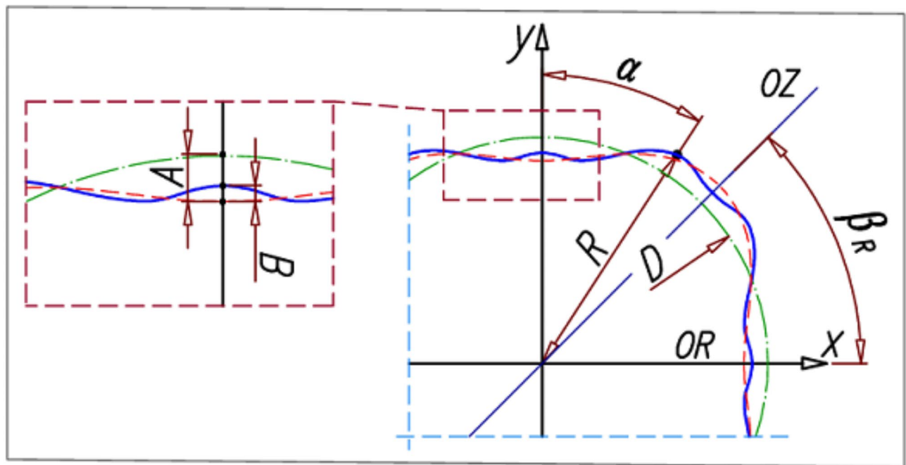
Fig. 4. Parameters of the rolling line of the rotor of the 4×6 type mechanism: OZ – axis of symmetry of the hump lift, OR – axis of symmetry of the hump rebate, D – diameter of the base circle of the rotor, A, B – amplitudes of the cosine function (formula (1)), R – radius of the rotor corresponding to the angle \alpha (formula (1)). (created in Autodesk Autocad 2024, https://www.autodesk.com/ )
