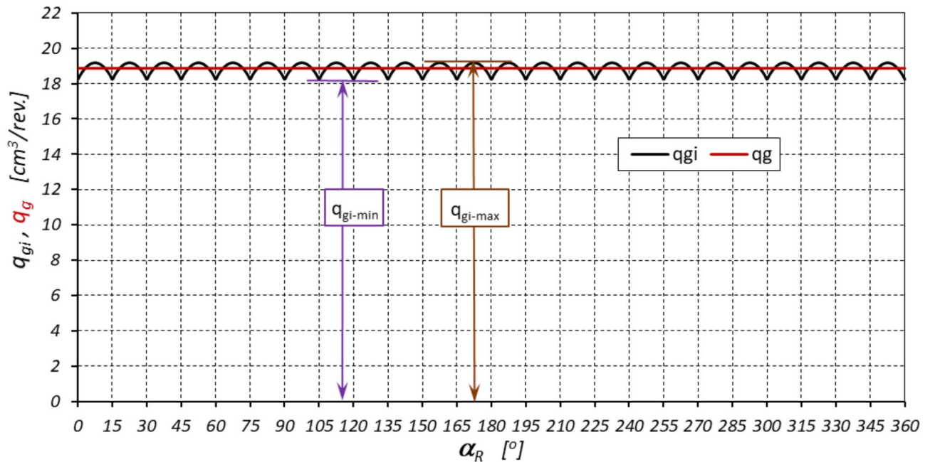
Fig. 15. Characteristics of the instantaneous geometric working volume q_{gi} and the average geometric working volume q_g of the satellite mechanism as a function of the angle of rotation \alpha_R of the rotor (within one complete rotation of the rotor – \alpha_R = 360^\circ ).
