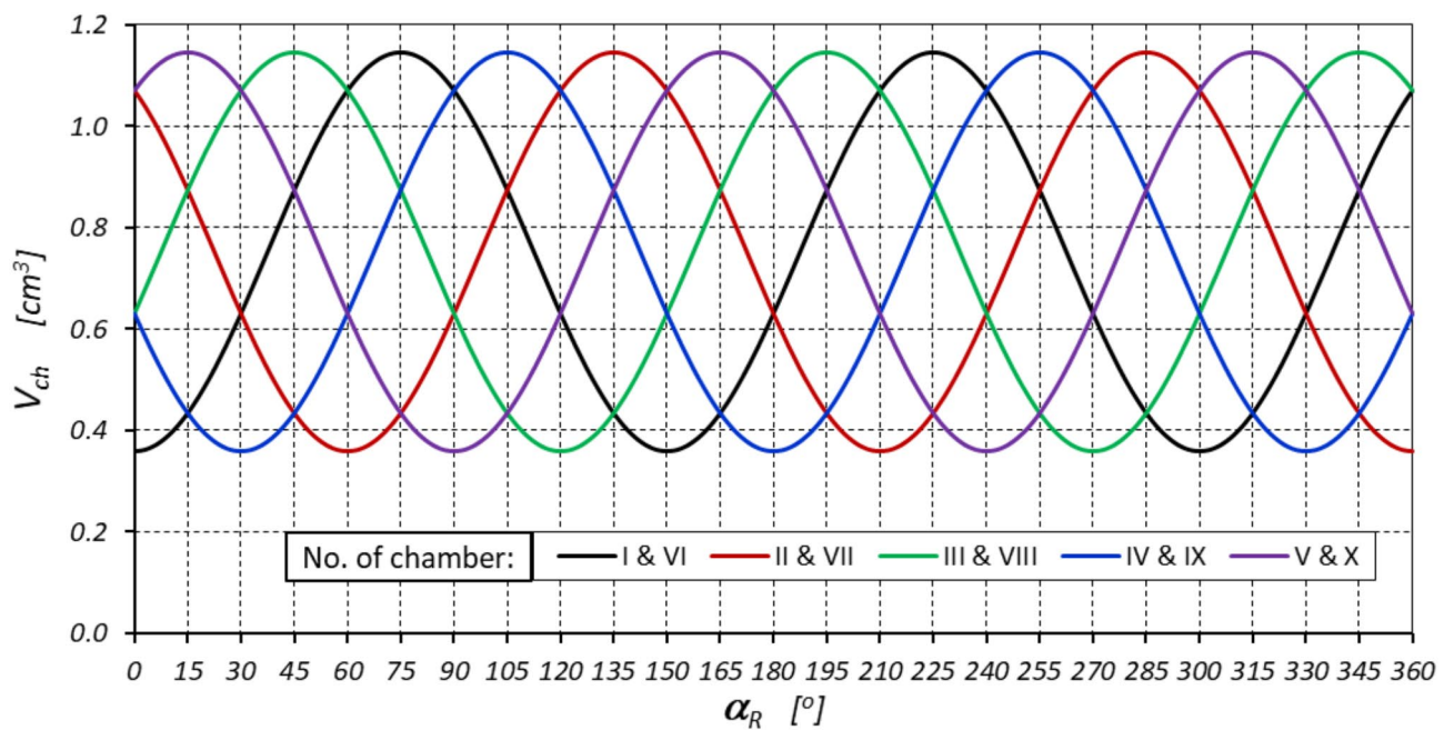
Fig. 6. Characteristics of the volume V_{ch} of the working chambers of the satellite mechanism as a function of the angle of rotation \alpha_R of the rotor (within one complete rotation of the rotor – \alpha_R = 360^\circ ).
