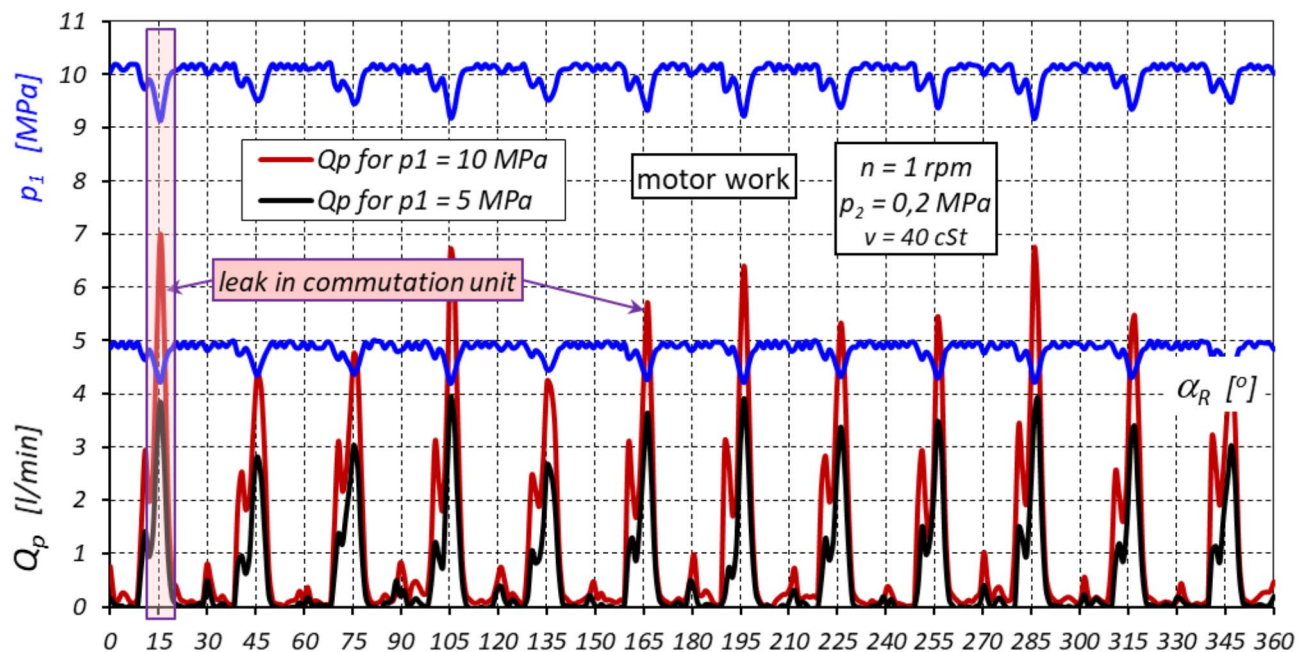
Fig. 31. Characteristics of the actual flow rate Q_p in the machine working as a motor as a function of the angle of rotation \alpha_R of the rotor (within one complete rotation of the rotor – \alpha_R = 360^\circ ). The pressure in the inflow port of the motor: p_1 = 5 MPa and p_1 = 10 MPa.
