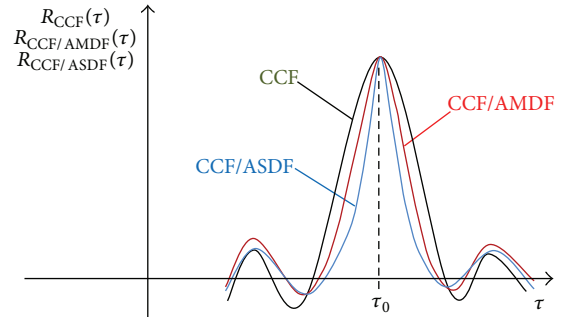
FIGURE 4: Exemplary view of combined CCF/AMDF and CCF/ASDF functions in comparison with CCF.
