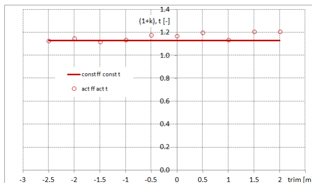
Figure 2. Form factor used in different methods
