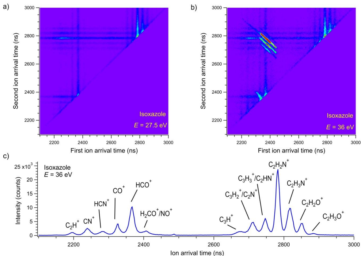
Figure 2. The coincidence maps of isoxazole measured at a) 27.5 eV and b) 36 eV. The vertical and horizontal stripes represent points where uncorrelated ions occurred. c) The time-of-flight mass spectrum of the cations detected at the 36 eV photon energy.
