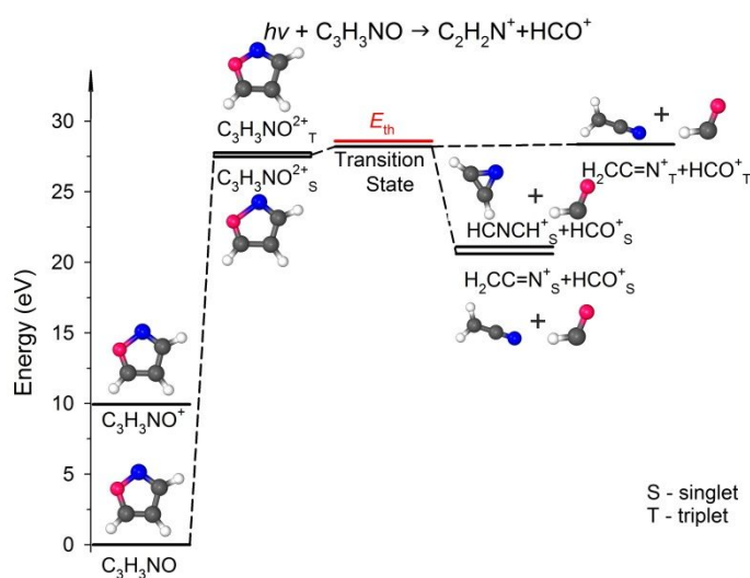
Figure 5. Relevant points in the potential energy surface of the isoxazole dication elucidating the HCO^+ + C_2H_2N^+ dissociation channel. The scheme is based on data presented in Table S1, ESI.
