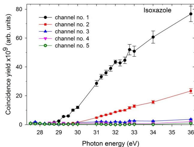
Figure 3. The coincidence yields of two-body dissociation channels following double photoionization of isoxazole in the 27.5-36 eV photon energy range (the assignments of the channels are given in Table 1).
