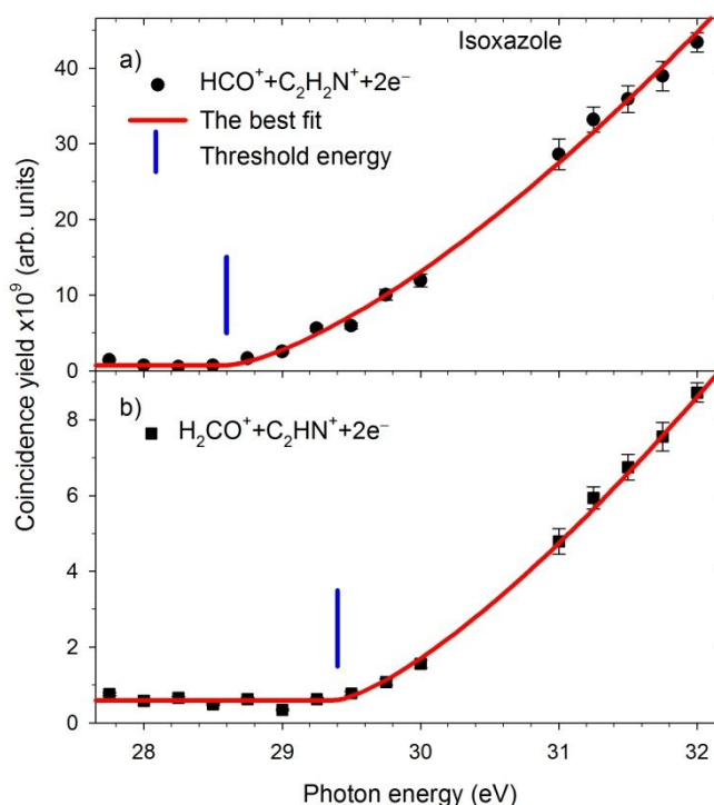
Figure 4. The yield curves of major dissociation channels measured in narrow energy regions near the expected AE thresholds. The solid red lines represent the best fits to the experimental data. The vertical blue bars show the energy positions of thresholds.
