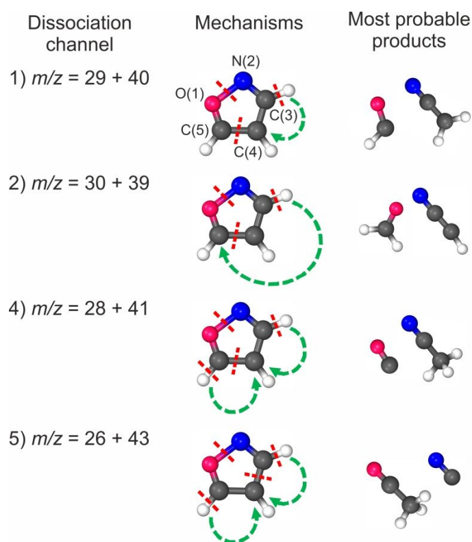
Figure 1. The courses of plausible dissociation channels that are accessible in the double photoionization of isoxazole. The numbers of the dissociation channels refer to those observed in the experiment (Section 3). Dissociation channel no. 3 is not shown here because it represents a heavy-isotope variant of dissociation channels 1 and 2 (see discussion in the text).
