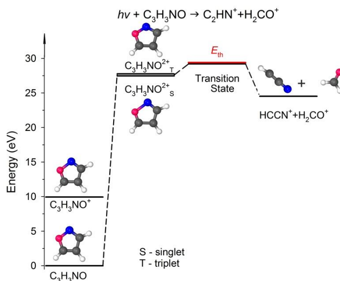
Figure 6. The simplified potential energy profile for the dissociation of the isoxazole dication into \text{H}_2\text{CO}^+ + \text{HCCN}^+ . The scheme is based on data presented in Table S1, ESI.
