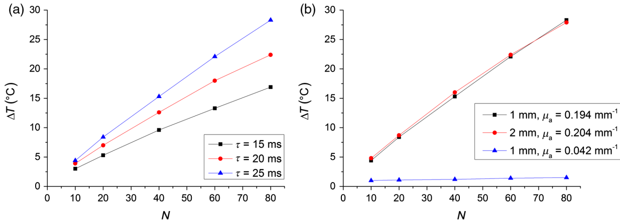
Fig. 3 Temperature increase as a function of the number of pulses N , at constant peak P = 10 W and T = 50 ms, (a) for different pulse widths \tau for 1-mm thick absorbing ( \mu_a = 0.194 \text{ mm}^{-1} ) phantom and (b) for different phantom thickness (frontal measurement) for pulse width \tau = 25 ms (b).
