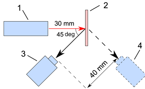
Fig. 2 Scheme of the measurement setup, consisting of: (1) a diode laser, (2) an optical skin phantom, (3) an infrared camera situated at “front” side, and (4) “backside” position. Distances between the elements of the set-up are shown. The red line denotes the laser beam at 975 nm, while the black lines represent the thermal radiation measured at 8 to 14 \mu\text{m} wavelength.
