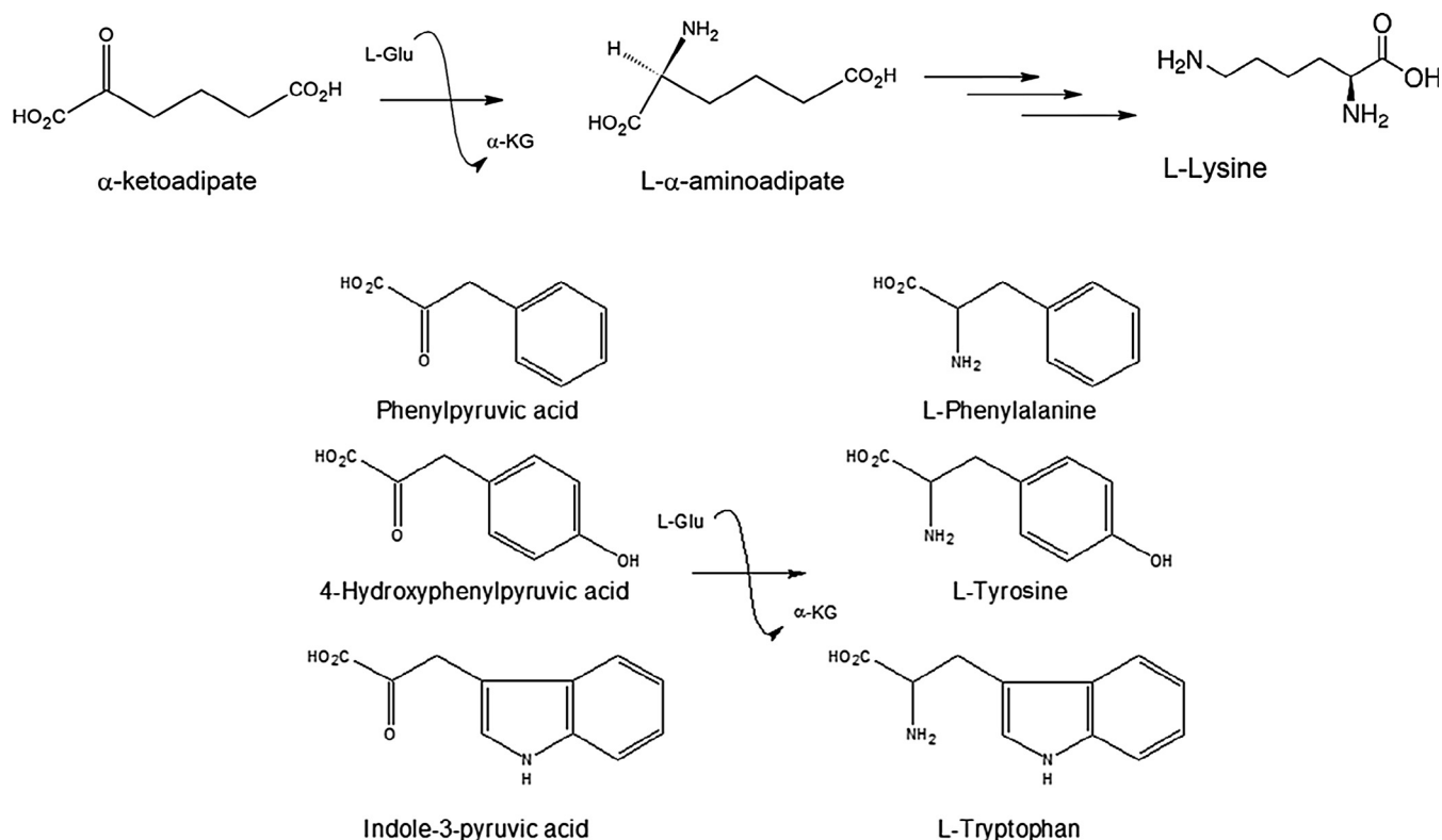
Fig. 1. The schematic overview of reactions performed by aromatic and aminoacidate transaminases for L-lysine and aromatic amino acids biosynthesis. The catabolic process is a reversal of the biosynthetic reaction.
