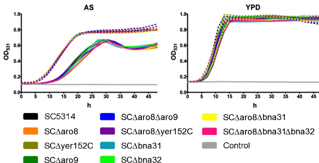
Fig. 6. Effect of (Aminoxy)acetate (AOA) on C. albicans wild-type and mutant growth in YNB with ammonium sulphate (AS) medium and YPD. Dashed lines, no AOA present; solid lines, 10 mM AOA. Optical density at 531 nm of the appropriate liquid medium served as a control.
