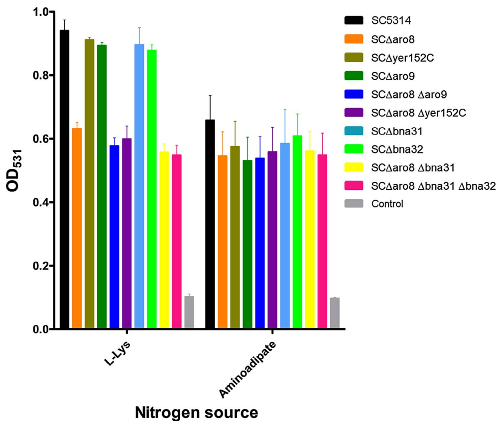
Fig. 4. Growth of C. albicans wild-type and deletion mutant strains in YNB media containing L-Lys or α-aminoacidate as the sole nitrogen source. Optical density of cell suspensions and liquid media (negative control) was measured at 531 nm after incubation for 48 h at 30 °C. All data represent the means ± SD.
